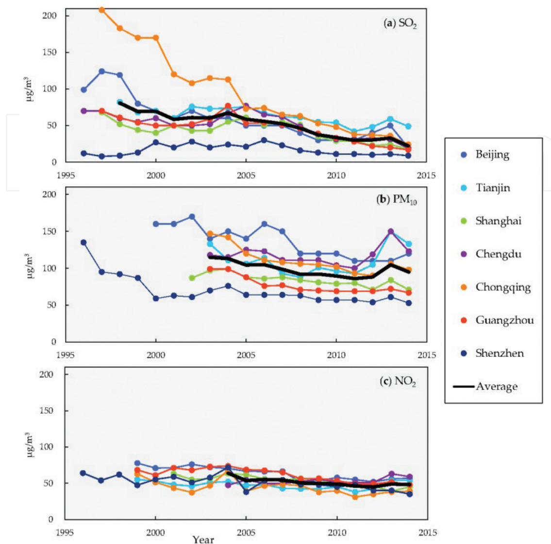
Figure 1. Trends of \text{SO}_2 (a); \text{PM}_{10} (b), and \text{NO}_2 (c) annual concentrations of seven China megacities in 1996–2014 (adopted from [11]).
