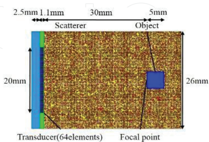
Figure 5. Simulation model for FDA compensation.
