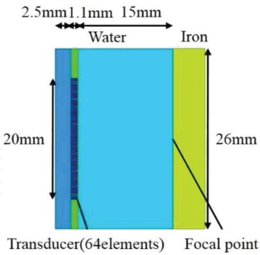
Figure 4. Simulation model for compensating transducer characteristics.
