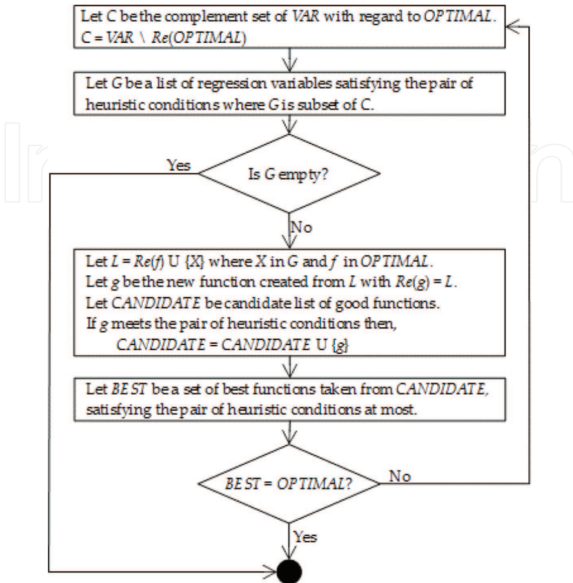
Figure 2. Flow chart of SG algorithm.
