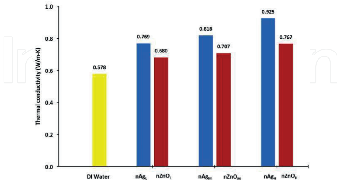
Figure 4. Thermal conductivity variation for silver and zinc oxide nanofluids with different volume fractions [16].
