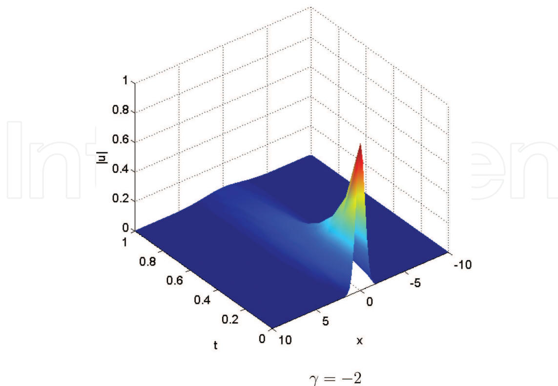
Figure 3. Numerical results for the nonlinear Ginzburg-Landau equation with \gamma = -2 in Example 4.2.
