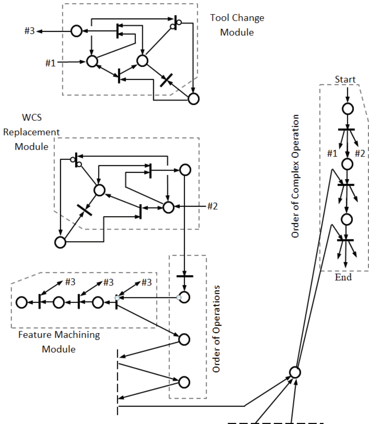
Figure 1. General (partial) multi-tool processing operation model.
