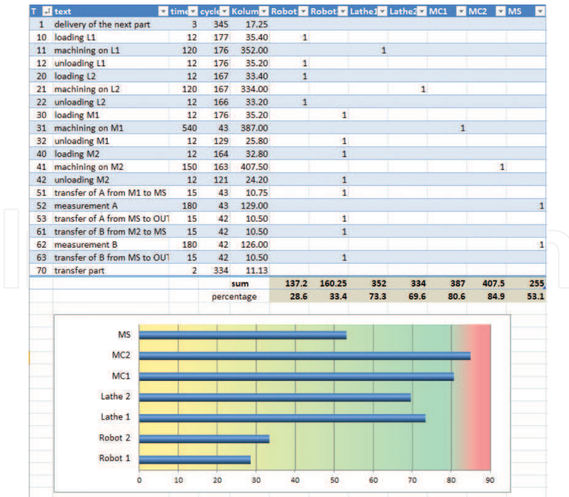
Figure 5. Spreadsheet of production resources utilization rate.
