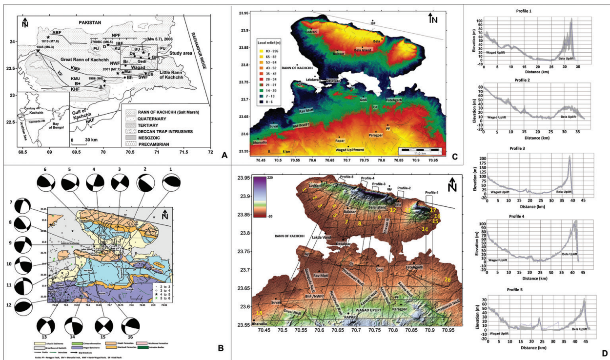
Figure 1. (A) Seismotectonic map of the Kachchh rift basin integrated with the geological map, showing the epicenters of significant earthquakes (modified after [10]). The Wagad area lies between the SWF and GF. Locations - A (Anjar), B (Bhuj), Ba (Bhachau), Br (Bharudia), Ch (Chitrod), D (Dholavira), De (Desalpar), L (Lakhpata), F (Fatehgarh) and G (Gedi); faults: NKF (North Kathiyawad Fault), KHF (Katrol Hill Fault), VF (Vigodi Fault), KMF (Kachchh Mainland Fault), SWF (South Wagad Fault), NWF (North Wagad Fault), GF (Gedi Fault), IBF (Island Belt Fault), ABF (Allah Bund Fault) and NPF (Nagar Parkar Fault); uplifts: KMU (Kachchh Mainland Uplift), PU (Patcham Uplift), KU (Khadir Uplift), BU (Bela Uplift), CU (Chorar Uplift). (B) Geological map of northern Wagad highland region [11]; shows location of earthquake epicenters. Focal mechanisms (1–16) plotted in the figure are after [12–15]. (C) CARTOSAT-DEM driven local relief map of Wagad Highland. Major and minor faults are marked by solid black line. (D) CARTOSAT DEM of the study area and location of the five swath profiles; 1–5) swath profiles show the trends of the maximum, minimum and mean topography of the Wagad region. Figure 1A and 1B have been digitized in Surfer 14 software, while, we used MICRO-DEM 10 software for generation of C and D, and final editing has been done in golden software Surfer 14.
