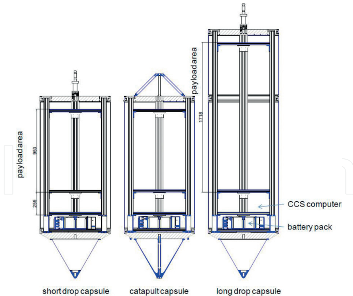
Figure 2. Different types and sizes of the drop capsule (photo: ZARM Drop Tower User Manual 2012).
