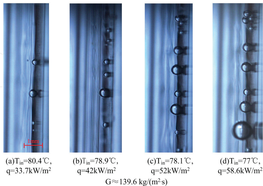
Figure 6. Typical sliding bubble with increasing heat flux.
