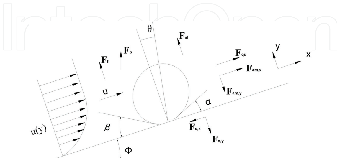
Figure 10. Force acting on a bubble.
