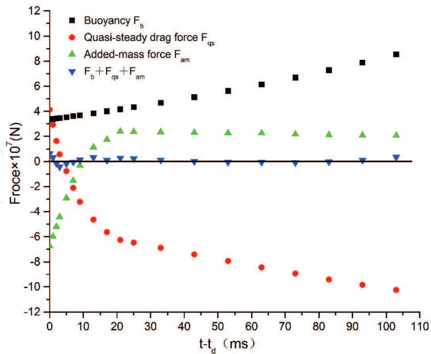
Figure 15. Force acting on the sliding bubble in inclined 45° upward facing upflow.
