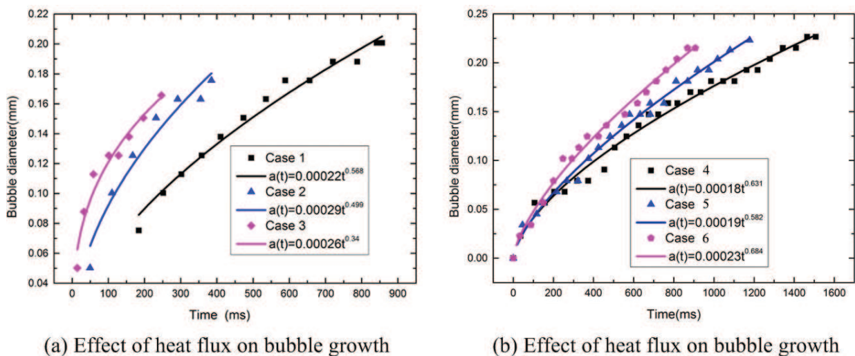
(a) Effect of heat flux on bubble growth Case1: G=140.3\text{kg/m}^2 \cdot \text{s} , T_{in}=77.3^\circ\text{C} , q=26.3\text{kW/m}^2 Case2: G=139.2\text{kg/m}^2 \cdot \text{s} , T_{in}=79.5^\circ\text{C} , q=31.1\text{kW/m}^2 Case3: G=137.7\text{kg/m}^2 \cdot \text{s} , T_{in}=78.7^\circ\text{C} , q=40.4\text{kW/m}^2 Case4: G=253.6\text{kg/m}^2 \cdot \text{s} , T_{in}=74.5^\circ\text{C} , q=46.3\text{kW/m}^2 Case5: G=252.8\text{kg/m}^2 \cdot \text{s} , T_{in}=74.4^\circ\text{C} , q=46.7\text{kW/m}^2 Case6: G=250.0\text{kg/m}^2 \cdot \text{s} , T_{in}=73.6^\circ\text{C} , q=56.5\text{kW/m}^2
