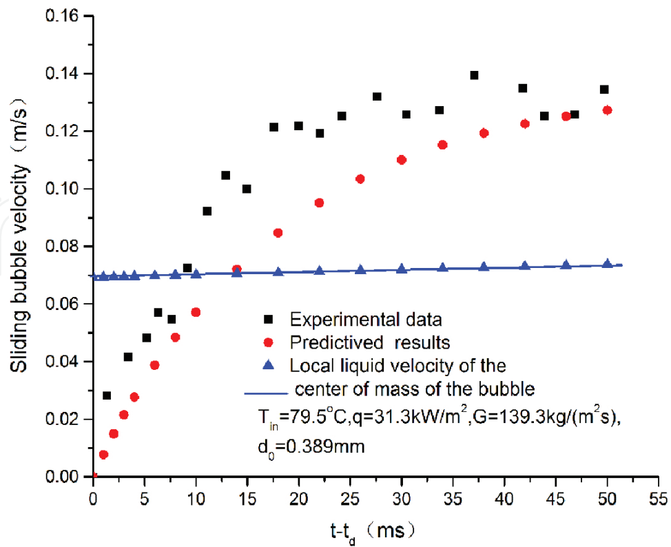
Figure 12. Sliding bubble velocity for vertical flow.
