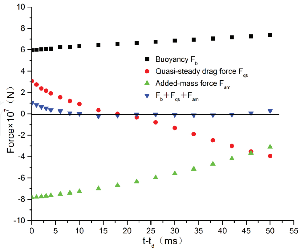
Figure 13. Forces acting on the sliding bubble for vertical flow.
