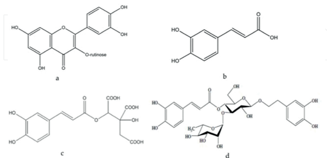
Figure 4. Structures of phytochemicals (a) quercetin-3-O-rutinoside, (b) caffeic acid, (c) Caffeoyl-hydroxycitric, and (d) verbascoside.
