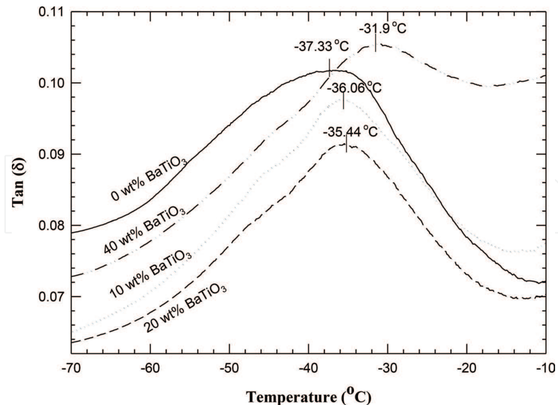
Figure 6. Plot of \tan \delta versus temperature obtained using DMA. The effect of BaTiO 3 content on the glass transition temperature ( T_g ) of the fiber is evaluated.
