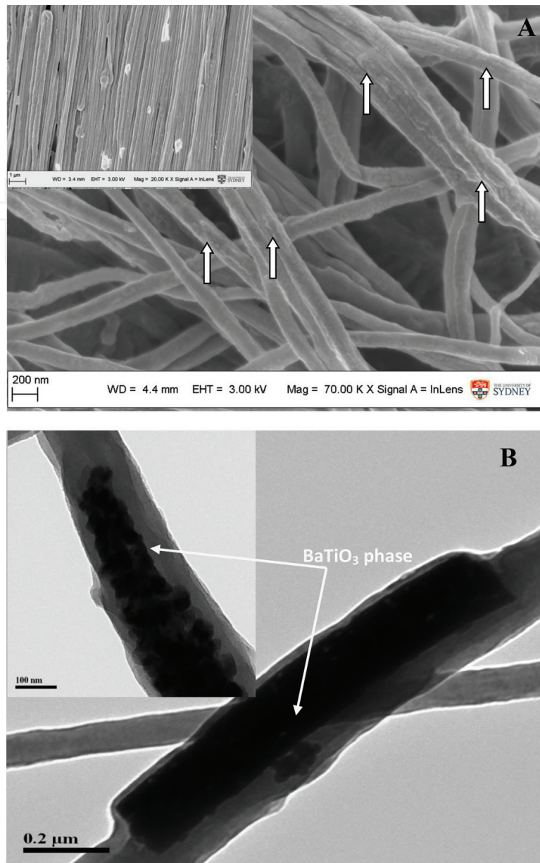
Figure 2. (A) SEM image of PVDF reinforced \text{BaTiO}_3 fibers (Sample 2). The inset in the figure shows the microstructure of uniaxially aligned fiber arrays. Aligned PVDF fibers as a function of \text{BaTiO}_3 content were collected for characterizing their tensile properties. (B) TEM images of typical PVDF fibers reinforced with 20 wt% \text{BaTiO}_3 . It is evident that the \text{BaTiO}_3 fiber is embedded within the PVDF matrix and aligned along its fiber axis. The inset in the figure shows a higher magnification image taken of another fiber area.
