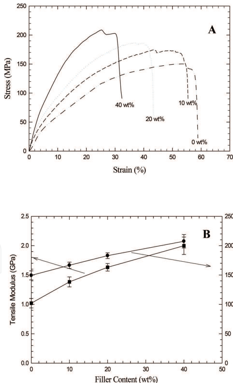
Figure 5. (A) Stress-strain curves obtained from tensile tests conducted on fiber samples as a function of BaTiO 3 concentration. (B) Plot of tensile strength and modulus of fiber samples as a function of BaTiO 3 content.
