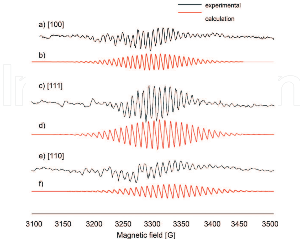
Figure 4. EPR spectra of the F-centers in the LiBaF3 crystal.
