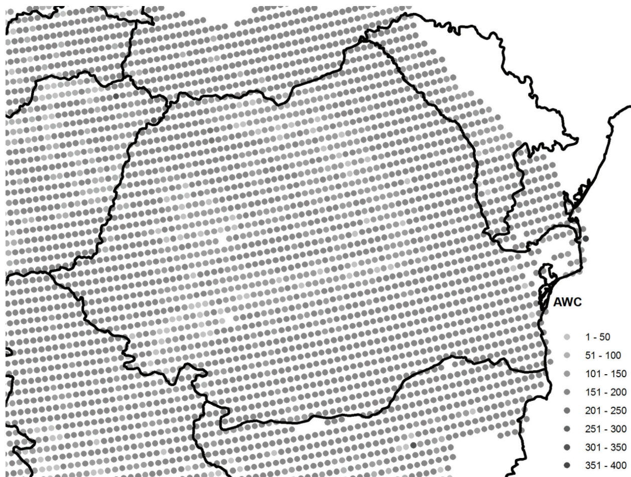
Figure 2. Available water capacities (AWCs) (in mm water column/1 m soil) computed in the 12.5 km EURO-CORDEX grids (black circles) obtained as the sum of topsoil and subsoil AWCs (at 1 km \times 1 km resolution) extracted from the European Soil Database (ESDB) and averaged over the 12.5 km \times 12.5 km grid cells centered in the model grids for the areas of interest.
