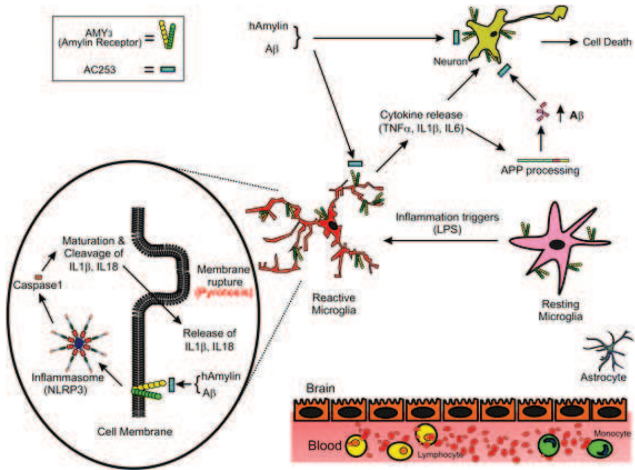
Figure 1. Model of neurodegeneration in AD proposed by Fu et al. [84]: Through the involvement microglia and neural amylin receptors in mediating the A\beta -induced neurodegeneration. Legend: The expression of amylin receptors of resting microglia, increased in response to inflammatory triggers like LPS, induces microglial cells activation. The interaction of A\beta with amylin receptors of the activated microglia leads to increased production and release of cytokines (TNF, IL-1 \beta , and IL-6), which act directly on neurons to produce cell death and additionally augment the production of A\beta via processing of the amyloid precursor protein (APP). The A\beta , in turn, interacts with neuronal and microglial amylin receptors to produce cell death. Adapted from Fu et al. [84]. Open access to this article is distributed under the terms of the creative commons attribution 4.0 international license ( http://creativecommons.org/licenses/by/4.0/ ), which permits unrestricted use, distribution, and reproduction in any medium, provided you give appropriate credit to the original author(s) and the source, provide a link to the creative commons license, and indicate if changes were made. The creative commons public domain dedication waiver ( http://creativecommons.org/publicdomain/zero/1.0/ ) applies to the data made available in this article, unless otherwise stated.
