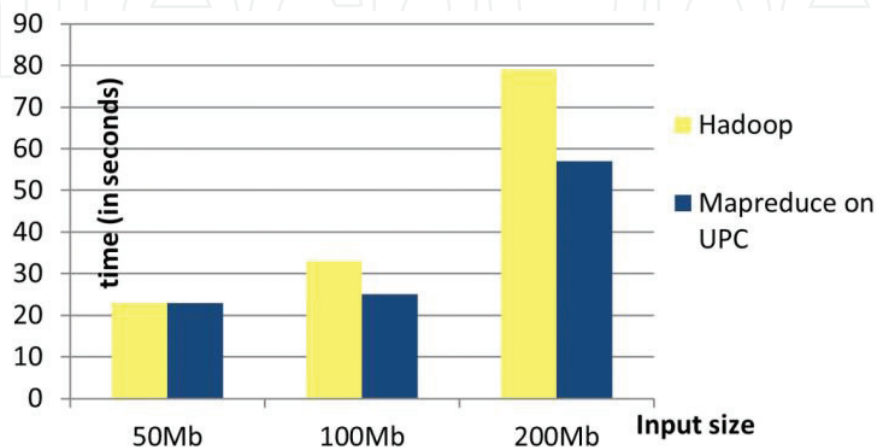
Figure 14. Apache Hadoop versus MapReduce on UPC.
