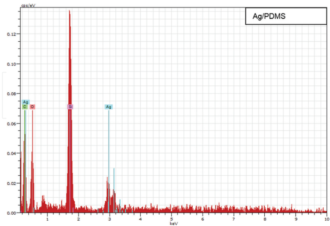
Figure 8. Silver nanoparticles immobilized on PDMS, Energy-dispersive X-ray spectroscopy (EDS) spectrum.
