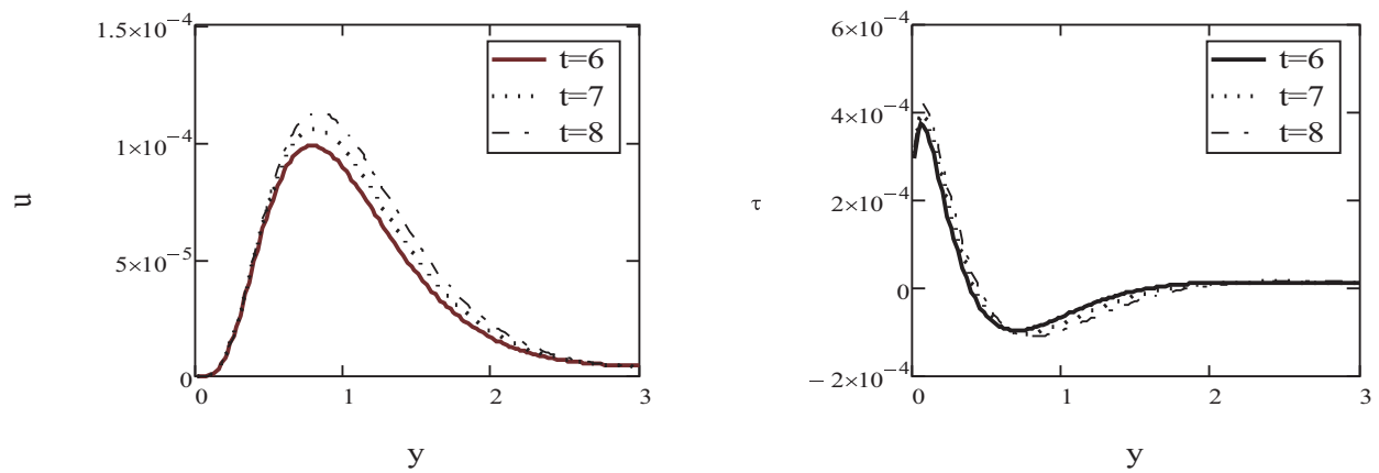
Figure 6. Velocity and shear stress profiles corresponding to the cosine oscillations of the duct for different values of t . Other parameters are taken as x = 0.5 , \lambda = 1.4 , U = 0.2 , H = 0.5 , K = 0.6 , d = 1 , h = 2 , \theta = 0.6 , \omega = 0.5 and \nu = 0.1 .
