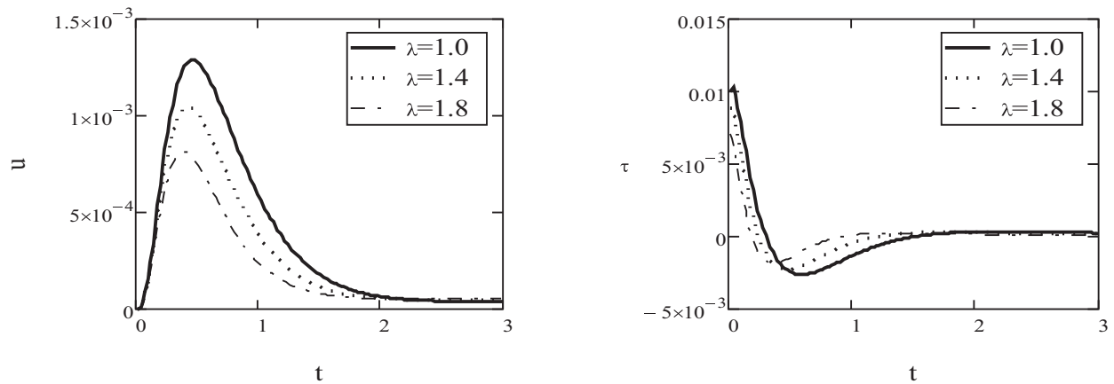
Figure 1. Velocity and shear stress profiles corresponding to the cosine oscillations of the duct for different values of \lambda . Other parameters are taken as x = 0.5, y = 0.3, U = 0.2, H = 0.5, K = 0.6, d = 1, h = 2, \theta = 0.6, \omega = 0.5 and \nu = 0.1 .
