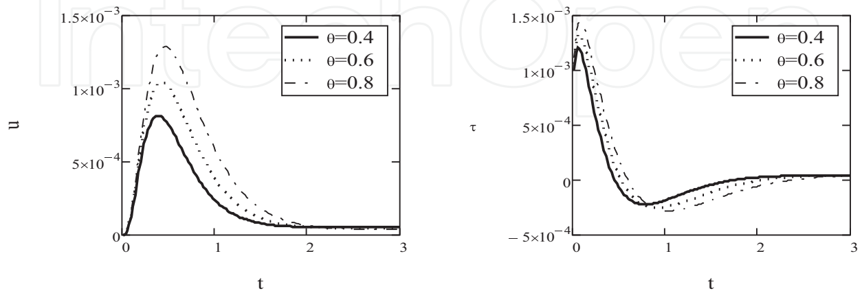
Figure 2. Velocity and shear stress profiles corresponding to the cosine oscillations of the duct for different values of \theta . Other parameters are taken as x = 0.5, y = 0.3, U = 0.2, H = 0.5, K = 0.6, d = 1, h = 2, \lambda = 1.4, \omega = 0.5 and \nu = 0.1 .
