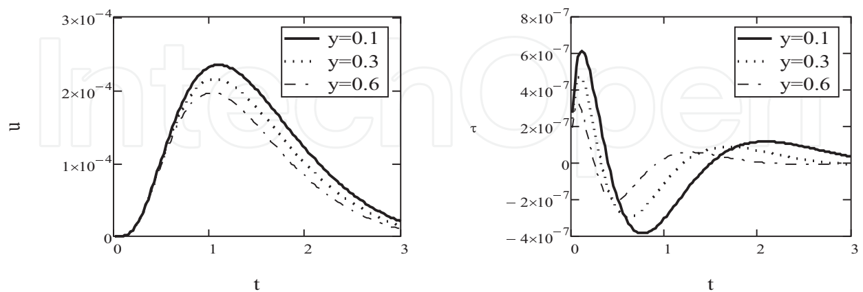
Figure 7. Velocity and shear stress profiles corresponding to the cosine oscillations of the duct for different values of y . Other parameters are taken as x = 0.5 , \lambda = 1.4 , U = 0.2 , H = 0.5 , K = 0.6 , d = 1 , h = 2 , \theta = 0.6 , \omega = 0.5 and \nu = 0.1 .
