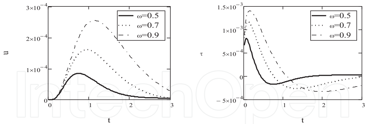
Figure 3. Velocity and shear stress profiles corresponding to the cosine oscillations of the duct for different values of \omega . Other parameters are taken as x = 0.5, y = 0.3, U = 0.2, H = 0.5, K = 0.6, d = 1, h = 2, \theta = 0.6, \lambda = 1.4 and \nu = 0.1 .
