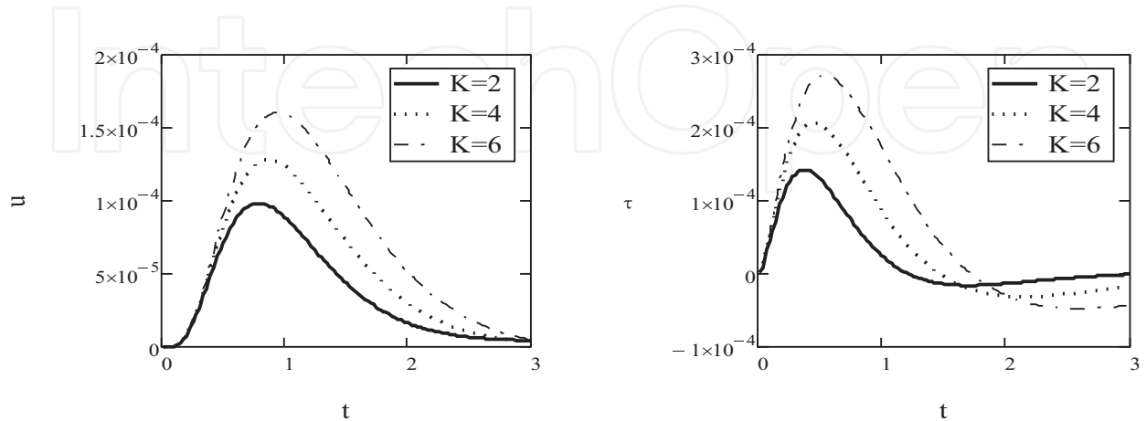
Figure 5. Velocity and shear stress profiles corresponding to the cosine oscillations of the duct for different values of K . Other parameters are taken as x = 0.5, y = 0.3, U = 0.2, H = 0.5, \lambda = 1.4, d = 1, h = 2, \theta = 0.6, \omega = 0.5 and \nu = 0.1 .
