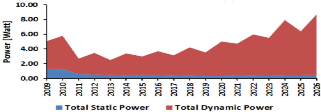
Figure 6. Power analysis chart, IRTS-2011.
