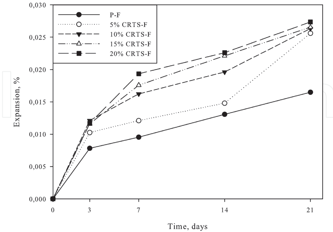
Figure 9. Improvement in ASR of the specimens without fly ash over 21 days.
