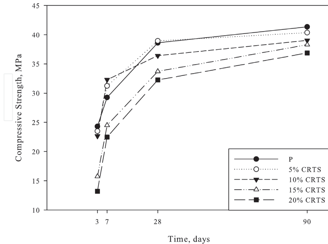
Figure 3. Improvement in compressive strength of the specimens over 90 days.
