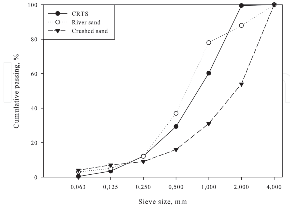
Figure 2. Particle size distributions of fine aggregates.
