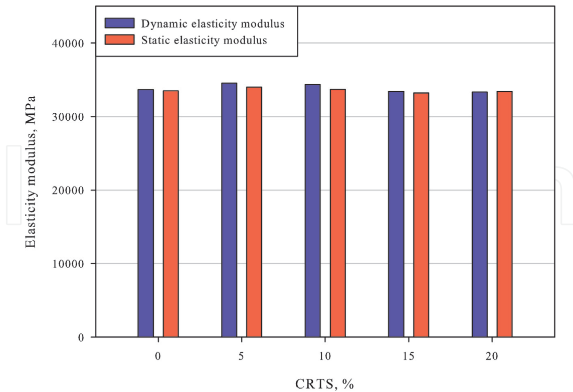
Figure 7. Static and dynamic elasticity moduli of the specimens at 28 days.
