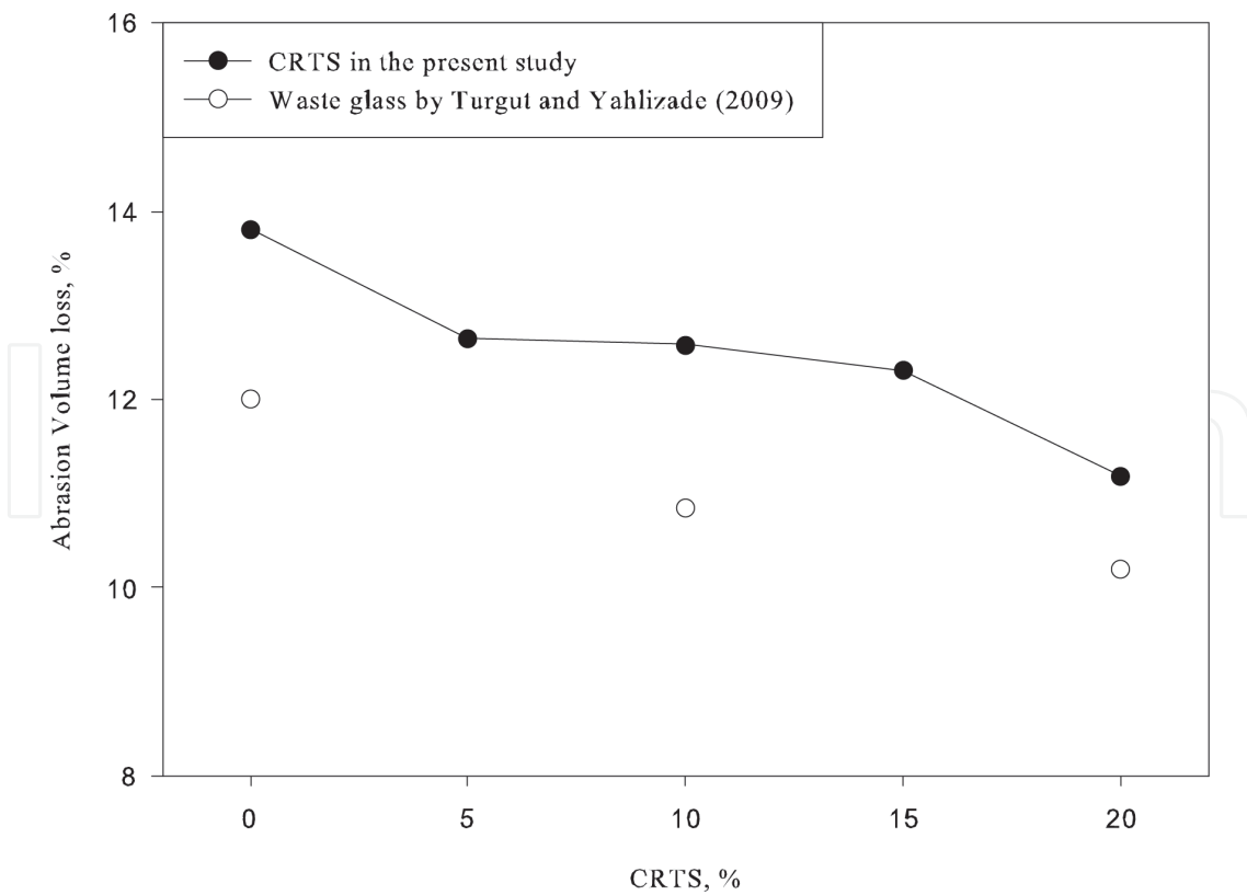
Figure 10. Change in abrasion loss (%) of the specimens after 28 days as a function of CRT comparing with the research by Turgut and Yahlizade.
