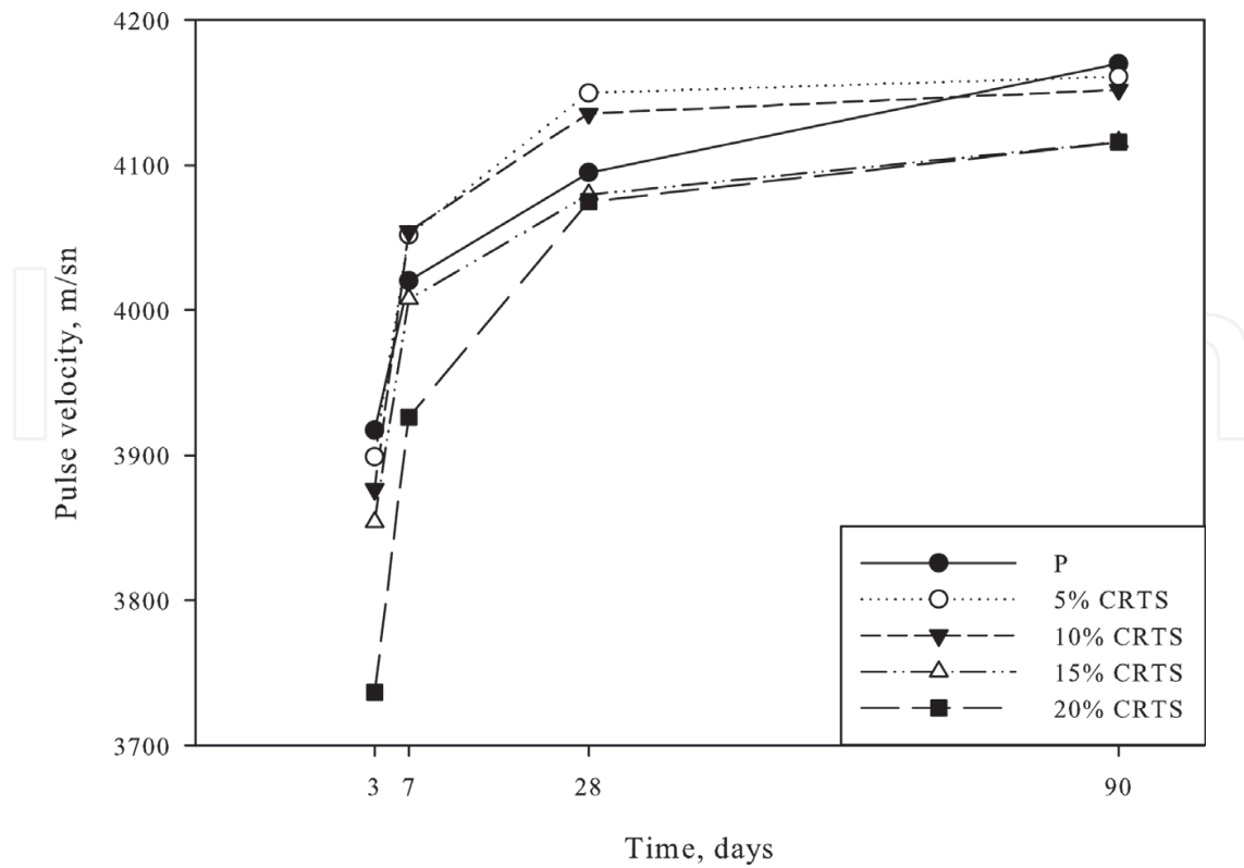
Figure 6. Improvement in ultrasonic pulse velocity of the specimens over 90 days.
