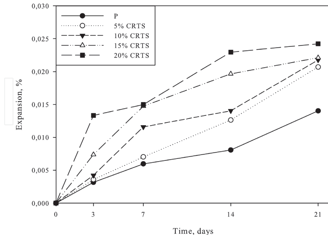
Figure 8. Improvement in ASR of the specimens over 21 days.
