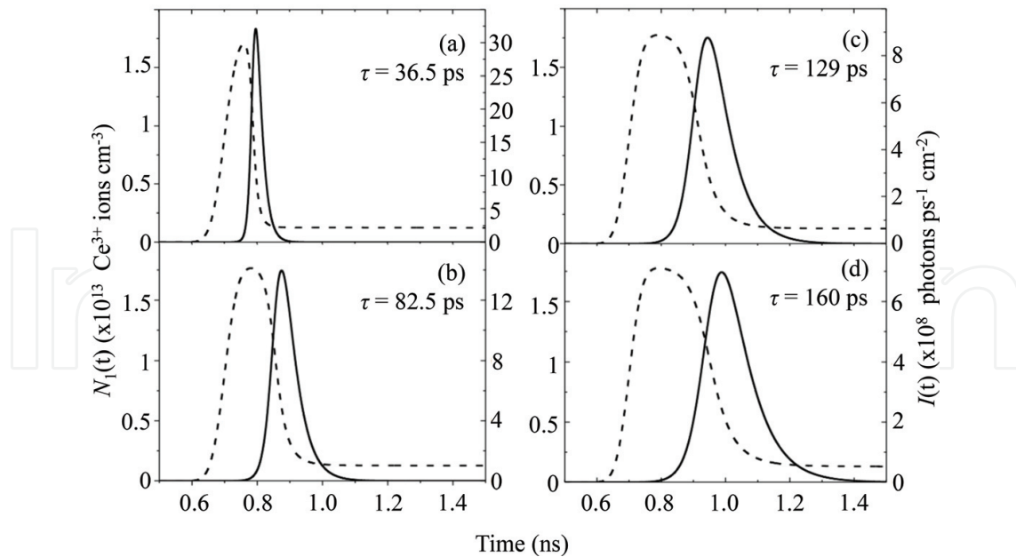
Figure 15. Temporal evolution of the Ce:LiCAF laser emission for different cavity lengths, L , of (a) 2 mm (b) 5 mm, (c) 8 mm, and (d) 10 mm. I(t) is represented by the solid plot while N_1(t) is represented by the dashed plot. The values of the following parameters that were kept constant are: N = 5 \times 10^{17} \text{ cm}^{-3} , l = 1 mm, R_1 = 100\% , R_2 = 30\% , r = 100 \mu\text{m} , \Delta t = 75 ps, n = 1.41 , and pump energy = 140 \mu\text{J} . The pump energy was chosen based on the effect of pump energy on pulse duration shown in Figure 16 .
