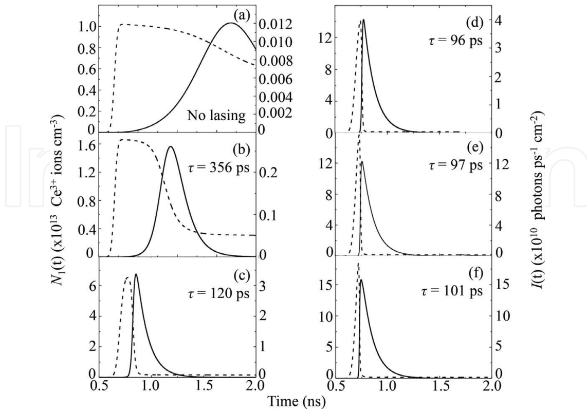
Figure 10. Temporal evolution of the Ce:LiCAF laser emission for different pump energies: (a) 25 \mu\text{J} , (b) 37.5 \mu\text{J} , (c) 150 \mu\text{J} , (d) 360 \mu\text{J} , (e) 450 \mu\text{J} , and (f) 600 \mu\text{J} . The dashed plot represents N_1(t) while the solid plot represents I(t) . The following parameters were kept constant: N = 5 \times 10^{17} \text{ cm}^{-3} , l = 10 \text{ mm} , L = 15 \text{ mm} , R_1 = 100\% , R_2 = 30\% , r = 100 \mu\text{m} , \Delta t = 75 \text{ ps} , and n = 1.41 .
