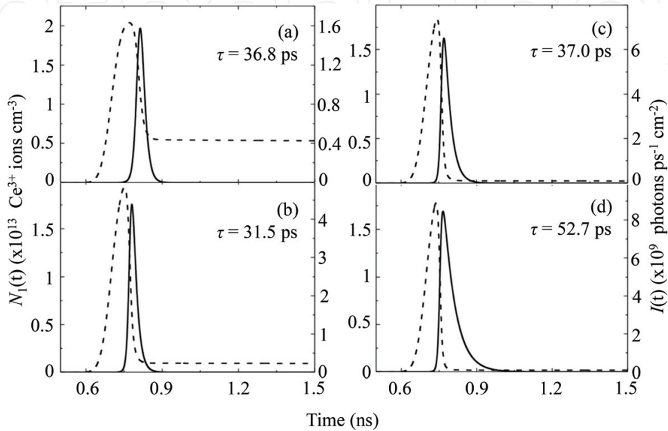
Figure 21. Temporal evolution of the laser emission for various output coupler reflectivity ( R_2 ). The length of the short Ce:LiCAF cavity oscillator is L = 2 mm. The various R_2 values considered are: (a) 10%, (b) 30%, (c) 50%, and (d) 70%. The following parameters were kept constant: N = 5 \times 10^{17} \text{ cm}^{-3} , l = 1 mm, R_1 = 100\% , \Delta t = 75 ps, r = 100 \mu\text{m} , n = 1.41 , and pumping energy is 140 \mu\text{J} . The pump energy was chosen based on results in Figures 19 and 20 . Solid graph represents I(t) while dashed graph represents N_1(t) .
