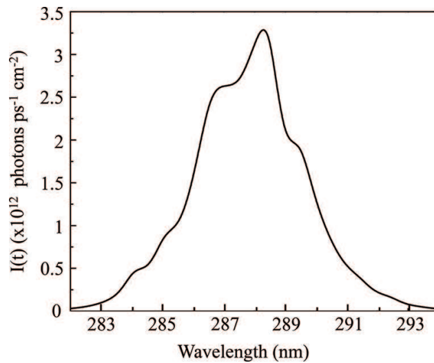
Figure 14. Spectral dynamics of the shortest achievable laser pulse duration (96 ps). The corresponding temporal dynamics is shown in Figure 10d .
