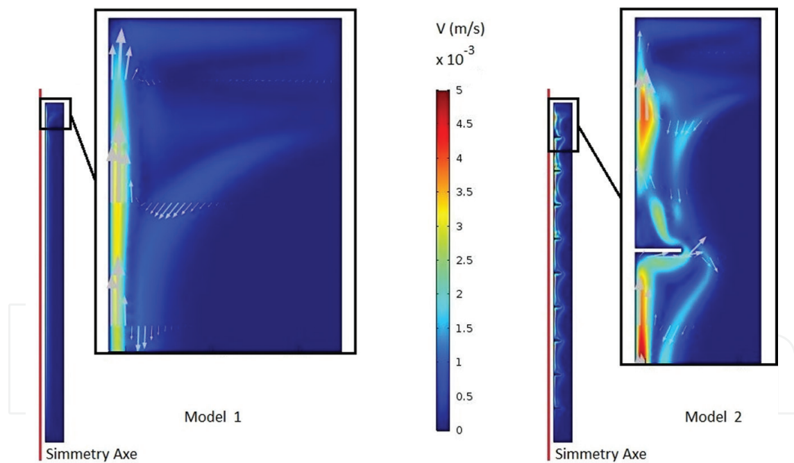
Figure 13. Velocity at t = 3900 s.
