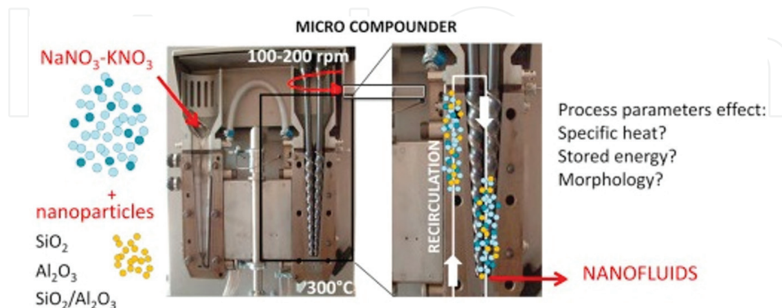
Figure 1. Mixing of nanoparticles and the salt mixture at high temperature in a twin screw microcompounder [21].
