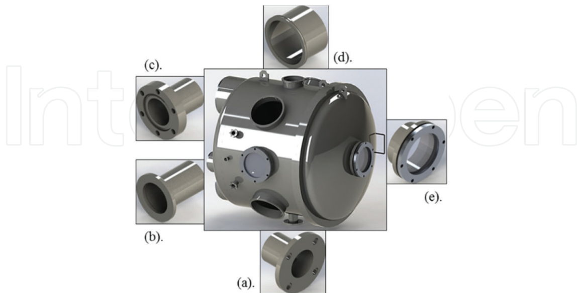
Figure 7. Common flange systems. (a) ASA flange, (b) KF flange, (c) CF flange, (d) ISO flange, (e) Viewport.
