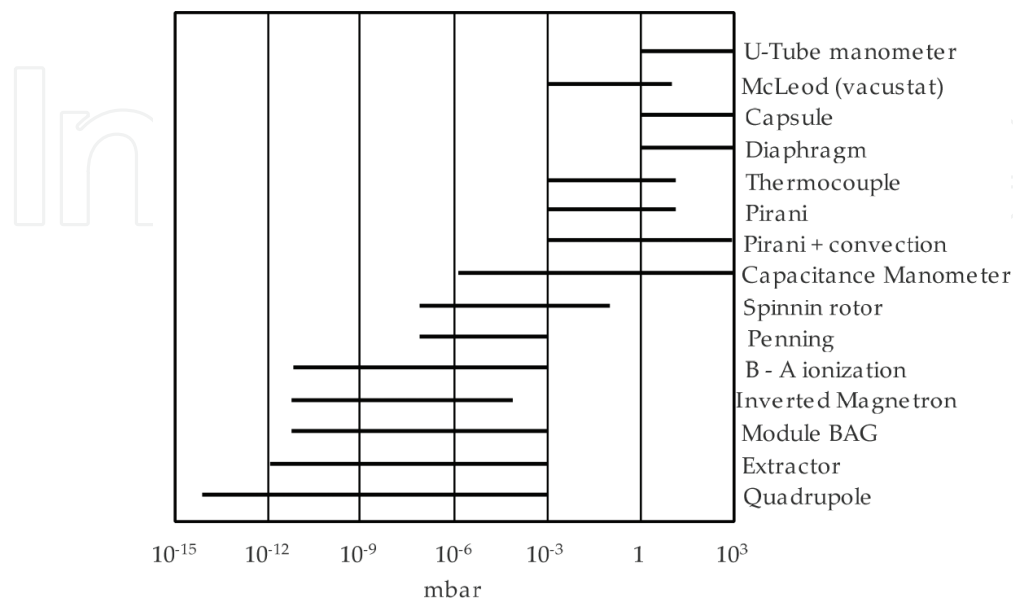
Figure 9. Pressure ranges for different gauges [14].
