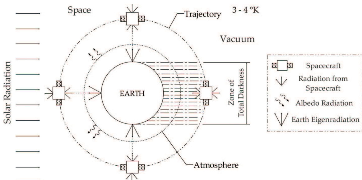
Figure 3. Space environment characteristics [3, 4].
