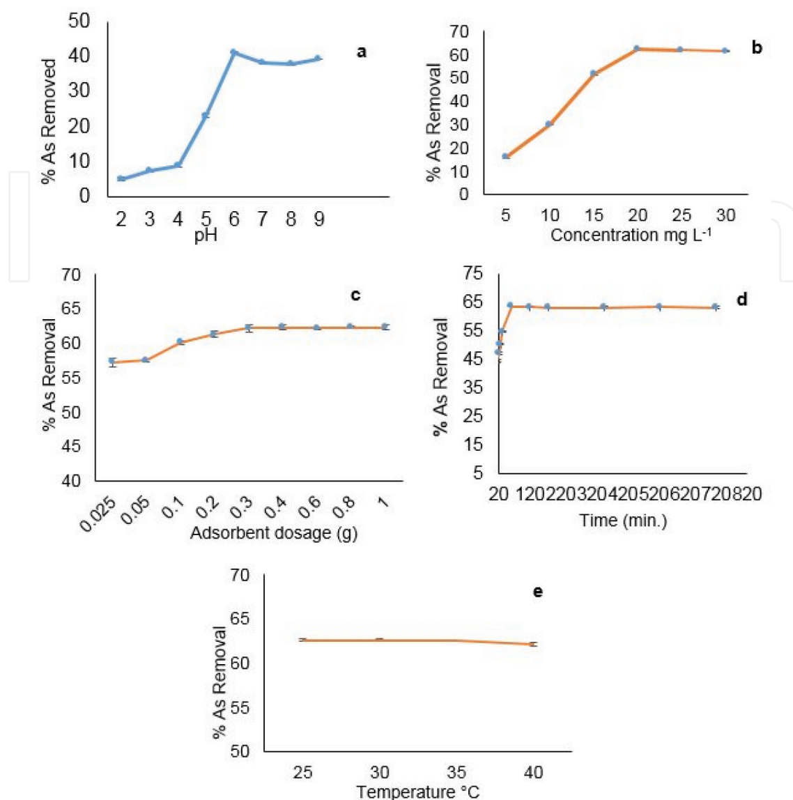
Figure 3. Optimization of (a) pH of the solution, (b) concentration of the analyte, (c) bio-adsorbent dosage, (d) contact time between the bio-adsorbent and the analyte, and (e) temperature of the solution.
