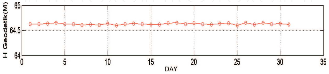
Figure 16. Repeatability of H result simulation baseline BNOA-CBTU 934,272.232 m.
