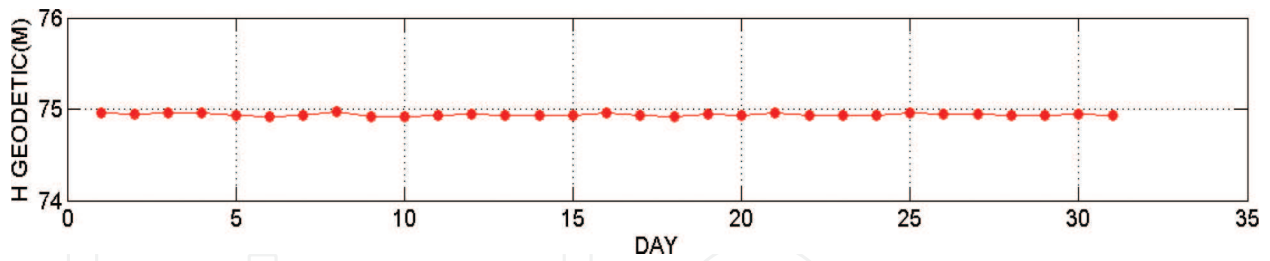
Figure 11. Repeatability of H result simulation baseline BAKO-BTNG 2,207,624.866 m.
