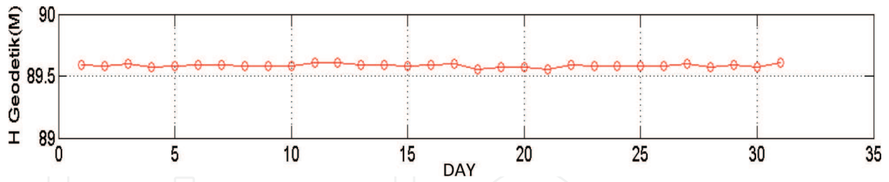
Figure 15. Repeatability of H result simulation baseline CNAB-CMAN 319,811.751 m.
