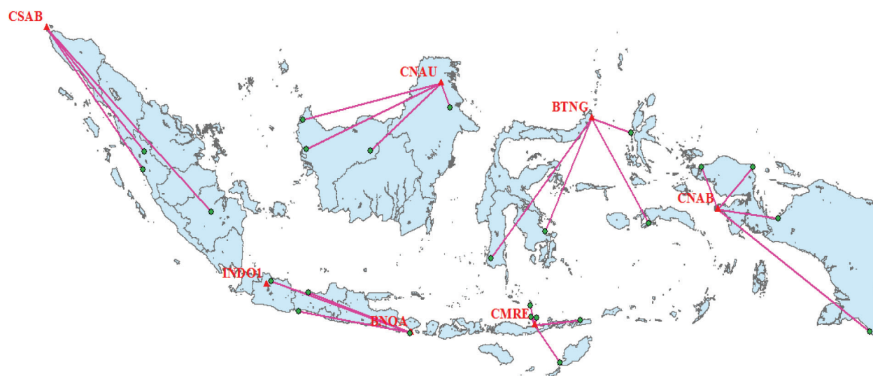
Figure 9. Baseline concepts using reference station at clustered offshore regions for subsidence monitoring around offshore oil and gas area of Indonesia.
