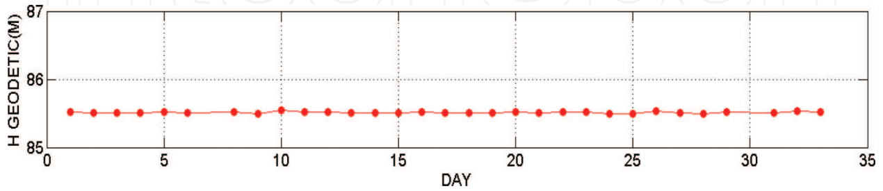
Figure 12. Repeatability of H result simulation baseline BAKO-CNAB 3,163,103.652 m.
