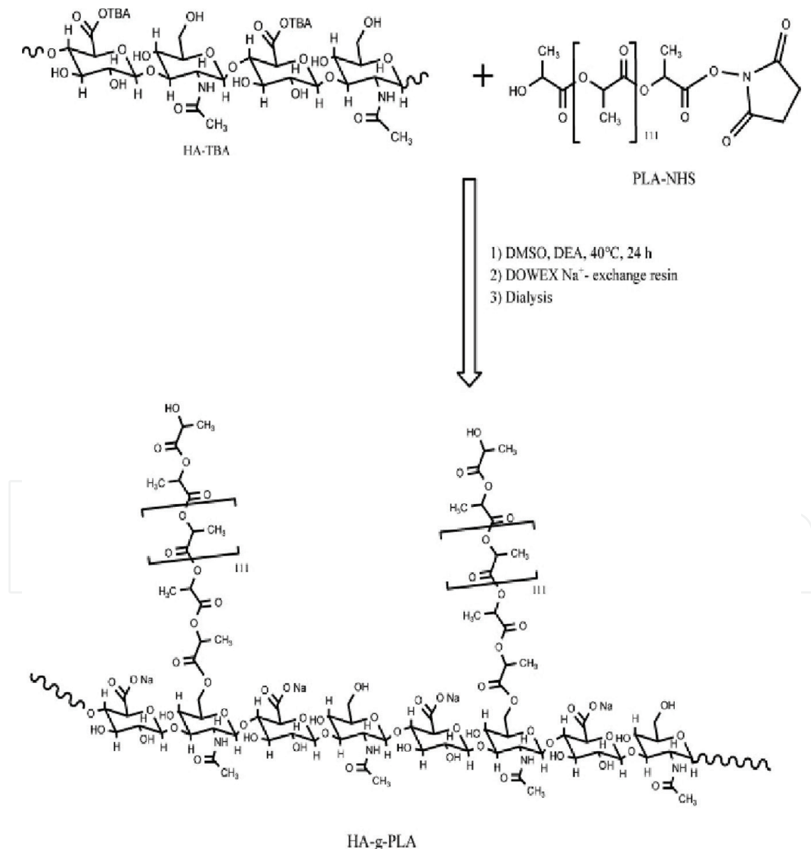
Figure 3. Principal steps in the synthesis of HA-g-PLA copolymer.
