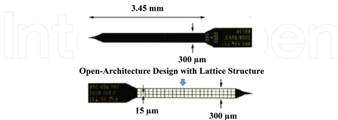
Figure 12. Comparison of a solid shank vs. the open-architecture design with a lattice structure. Reproduced from [25].
