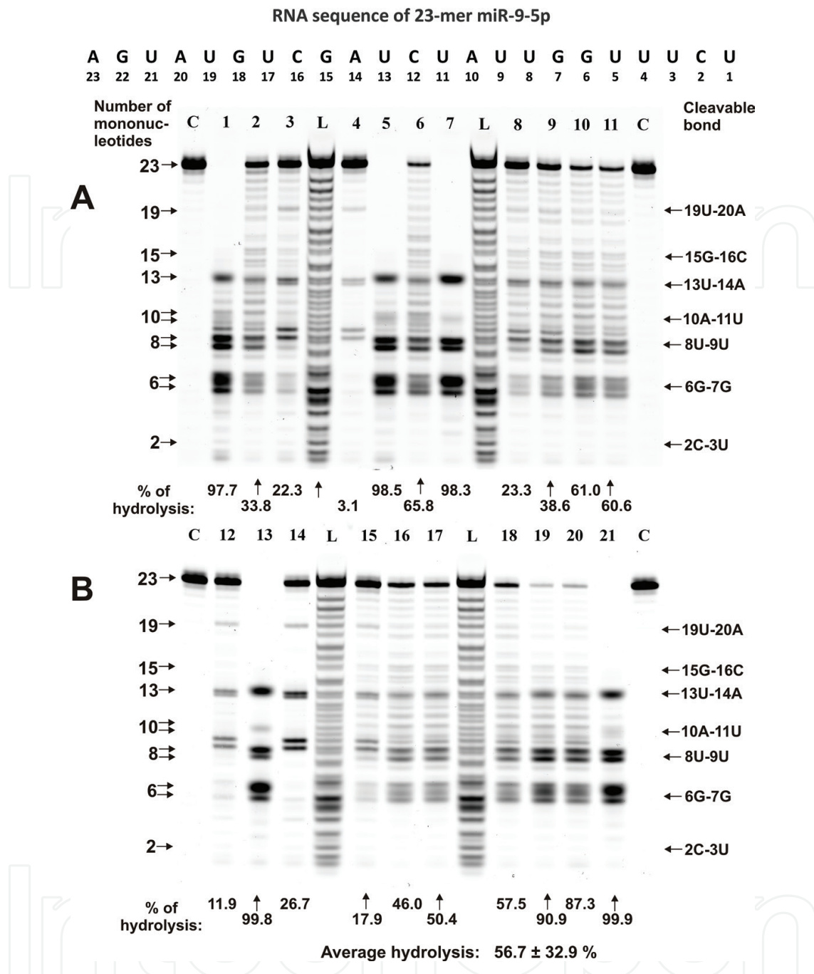
Figure 6. The patterns of Flu-miR-137 (0.01 mg/ml) hydrolysis by IgGs (0.1 mg/ml) from sera of 21 different SCZ patients. The hydrolysis products were detected by their fluorescence due to the fluorescent residue (Flu) on their 5'-ends. The numbers of antibodies, lengths of the products, and the percentage of microRNA hydrolysis by each preparation are indicated in panels A and B.
