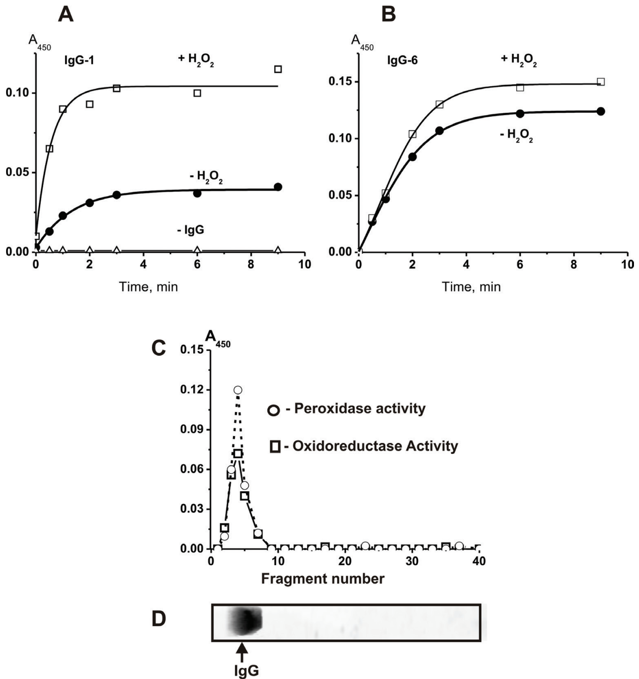
Figure 12. Typical kinetic curves of accumulation of a colored product ( A_{450} ) after DAB substrate oxidation by IgGs with peroxidase (in the presence of H_2O_2 ) (A) and with oxidoreductase (in the absence of H_2O_2 ) (B); activities in the oxidation of 3,3'-diaminobenzidine (0.2 mg/ml) in the case of 670 nM IgG-1 and IgG-6. Curve - IgG corresponds to the oxidation of the substrate in the absence of IgGs. SDS-PAGE analysis of peroxidase (○) and oxidoreductase (□) activities of IgG_{mix} (20 \mu g) (C and D). After electrophoresis, the 4–15% gradient gel was treated using special conditions for renaturation of IgG_{mix} . The RAs were evaluated using extracts of 40 gel fragments (2–3 mm); 20 \mu l of extracts were added to the standard mixtures and incubated for 24 h. The second band of the same gel was used to determine the position of intact IgG_{mix} (D); the gel was stained with Coomassie R250.
