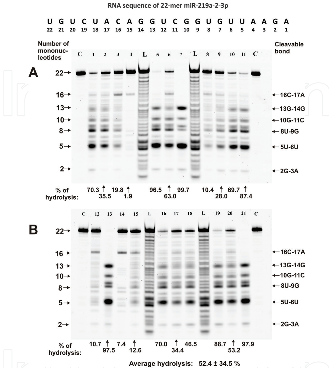
Figure 7. The patterns of Flu-miR-219a-2-3p (0.01 mg/ml) hydrolysis by IgGs (0.1 mg/ml) from sera of 21 different SCZ patients. The hydrolysis products were detected by their fluorescence due to the fluorescent residue (Flu) on their 5'-ends. The numbers of antibodies, lengths of the products, and the percentage of microRNA hydrolysis by each preparation are indicated in panels A and B.
