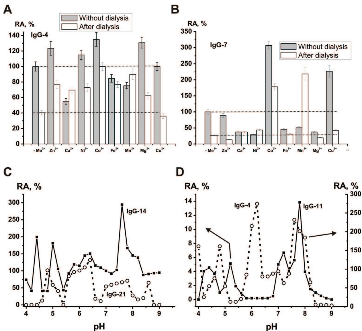
Figure 11. Effect of the dialysis of IgGs against EDTA for two individual scz-IgGs and different metal ions on the relative activity (RA, %) of dialyzed and non-dialyzed preparations (A and B). The RA of every non-dialyzed preparation was taken for 100%. Dependencies of the relative catalase activity of scz-IgGs on pH of the reaction mixture (C and D). All RAs of Abs before its preincubation were taken for 100%. The relative activity of IgG-14 at pH 7.0 was taken for 100%. All IgG preparations, metal ions, and conditions used marked on panels A–D. The errors in the determination of initial rate from three experiments in each case did not exceed 7–10%.
