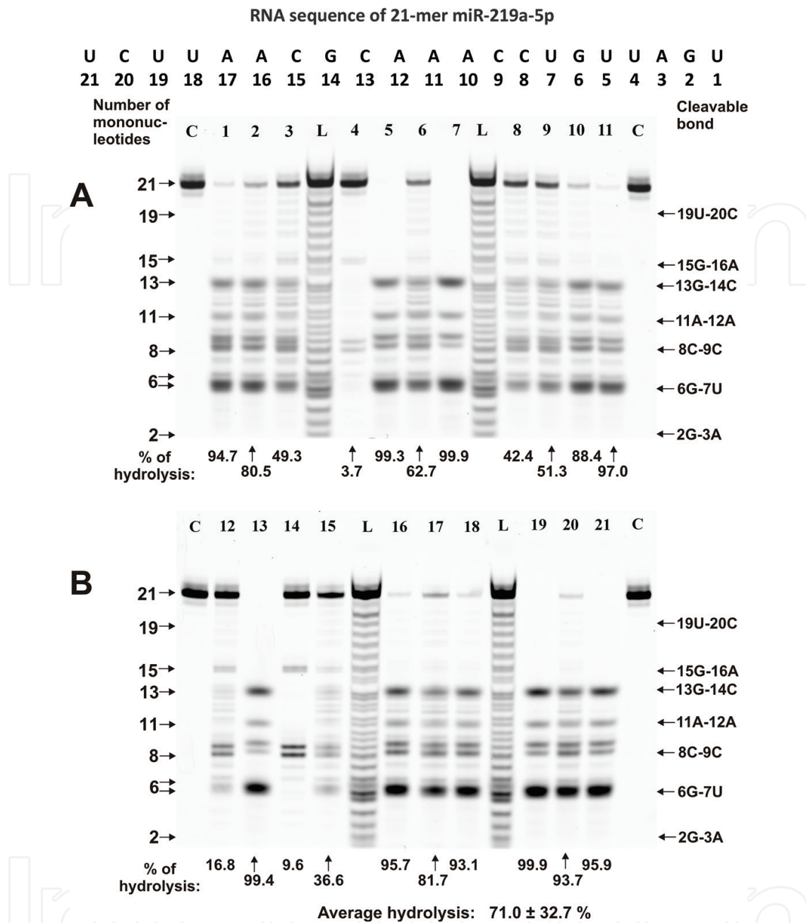
Figure 4. The patterns of flu- miR-219a-5p (0.01 mg/ml) hydrolysis by IgGs (0.1 mg/ml) from sera of 21 SCZ patients. The hydrolysis products were detected by their fluorescence due to the fluorescent residue (flu) on their 5'-ends. The numbers of antibodies, lengths of the products, and the percentage of microRNA hydrolysis by each preparation are indicated in panels A and B.
