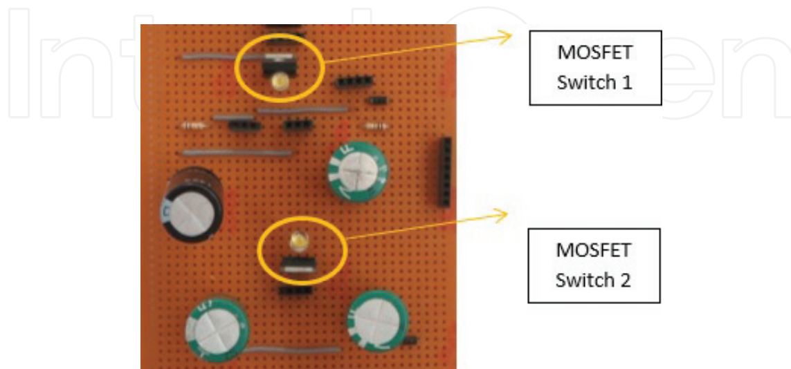
Figure 4. MOSFET configurations in energy harvesting circuit.
