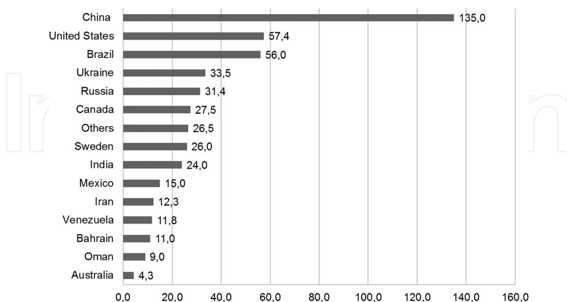
Figure 1. World installed pelletizing capacity (millions of tons/year). Source: Prepared by the authors with data from Tuck and Virta [2].
