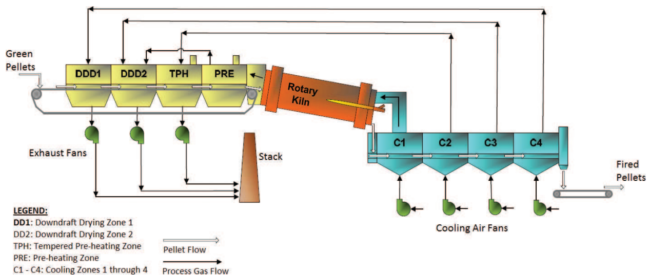
Figure 8. Schematic diagram of the grate-kiln induration process [29].
