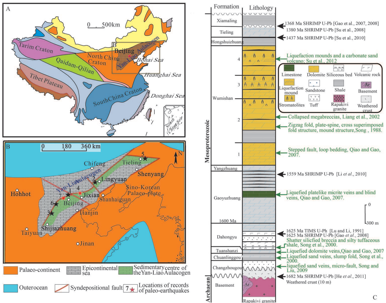
Figure 12. (A) Paleogeographic sketch map of China, showing the distribution of the major paleo-plates of different ages (after [62]). (B) Paleogeographic map of the Yan-Liao Aulacogen from the Proterozoic Gaoyuzhuang Stage to the Wumishan Stage showing an epicontinental sea opened to the north, and the approximate positions of the discovered seismicites (after [63–66]). The identified outcrops of earthquake-triggered SSDs are marked by stars, 1–[60]; 2–[67]; 3–[68]; 4 and 5–[64]; 6–[32, 69]; 7–[66]. The red stars show the position of the seismicites in this paper. (C) Lithostratigraphy of the Mesoproterozoic of the Yan-Liao Aulacogen (modified from [66–74, 77–79]), the records of multiple paleo-earthquake events in green words and volcanic events in black words are shown.
