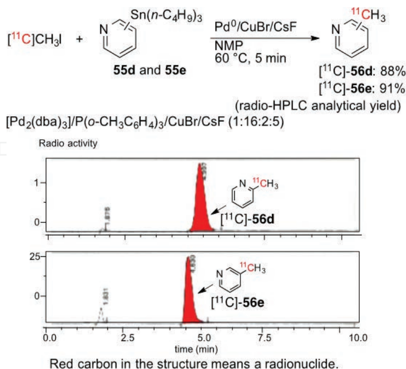
Figure 12. Syntheses of 2- and 3- [\text{C}^{11}] methylpyridines ( [\text{C}^{11}\text{]-56d and [\text{C}^{11}\text{]-56e ).
