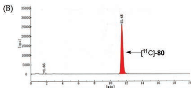
Figure 19. Synthetic scheme of ^{11}\text{C} -labeled p -xylene ( [^{11}\text{C}]\text{-80} ) by rapid C- [^{11}\text{C}] methylation using p -tolueneboronic acid pinacol ester (79) (A), and radio-HPLC chart in the analysis of the reaction mixture (B).
