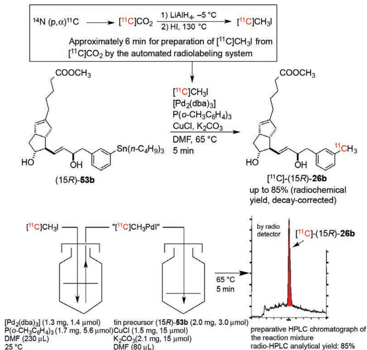
Figure 10. Synthesis of 15R- [^{11}\text{C}] TIC methyl ester ( [^{11}\text{C}]\text{-(15R)-26b} ) using a two-pot stepwise procedure.
