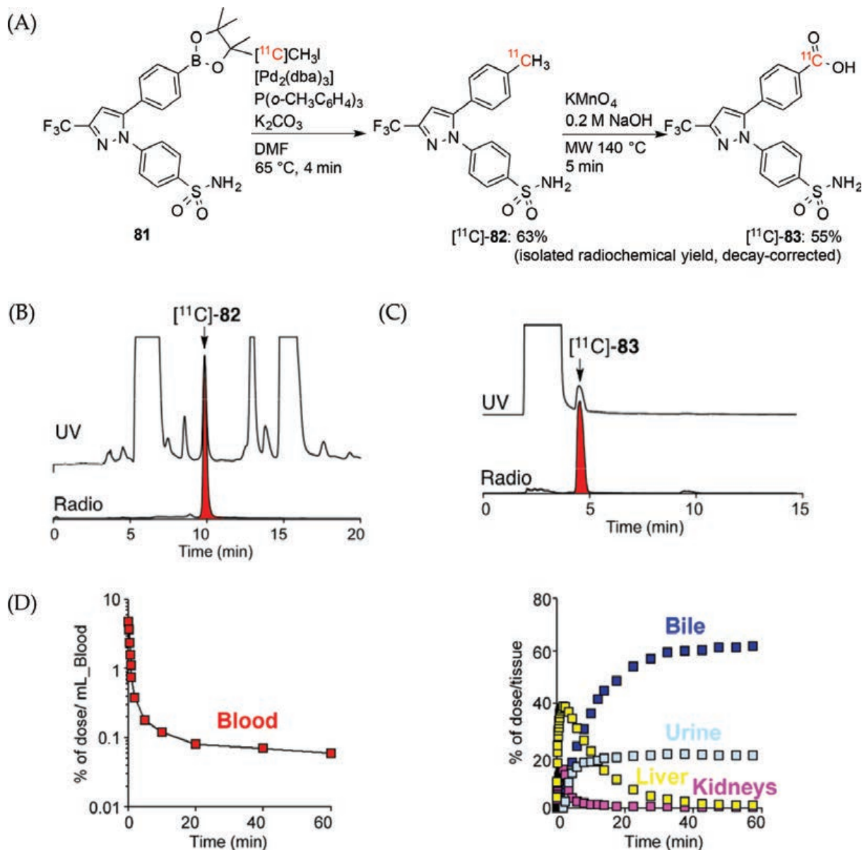
Figure 20. Syntheses of [^{11}\text{C}] celecoxib ( [^{11}\text{C}]\text{-82} ) and [^{11}\text{C}]\text{JC-62807} ( [^{11}\text{C}]\text{-83} ) (A), radio-HPLC analyses of [^{11}\text{C}]\text{-82} (B) and [^{11}\text{C}]\text{-83} (C), and the time profiles of the radio activity of [^{11}\text{C}]\text{-83} in the blood (red point), liver (yellow point), kidney (pink point), bile (blue point), and urinary bladder (light blue point) determined by PET imaging studies and blood sampling over a 60-min period after administration of [^{11}\text{C}]\text{-83} to male Sprague-Dawley rats (D). The peaks at retention times of 9.6 (in B) and 4.4 min (in C) are [^{11}\text{C}]\text{-82} and [^{11}\text{C}]\text{-83} , respectively. UV absorbance: 254 nm.
