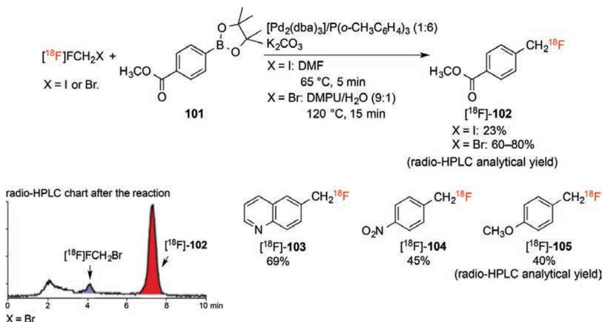
Figure 25. Rapid C- ^{18}\text{F} fluoromethylation of an arylboronic acid pinacol ester ( 101 ) with ^{18}\text{F} CH _2 X (X = I or Br).
