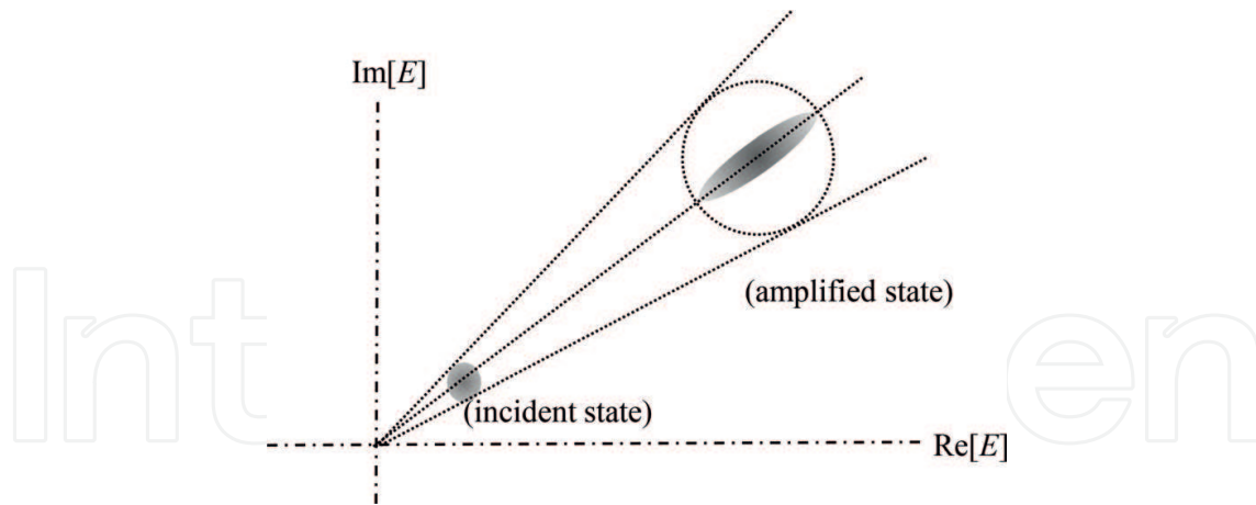
Figure 3. Constellation diagram of amplified light in a phase-synchronized degenerate OPA.
