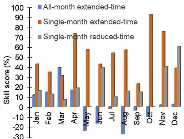
Figure 3. Skill scores for monthly forecasts for Victoria Mill (central Queensland), including the comparison between single-month optimization for short duration (reduced-time) and long duration (extended-time) forecasts [20].
