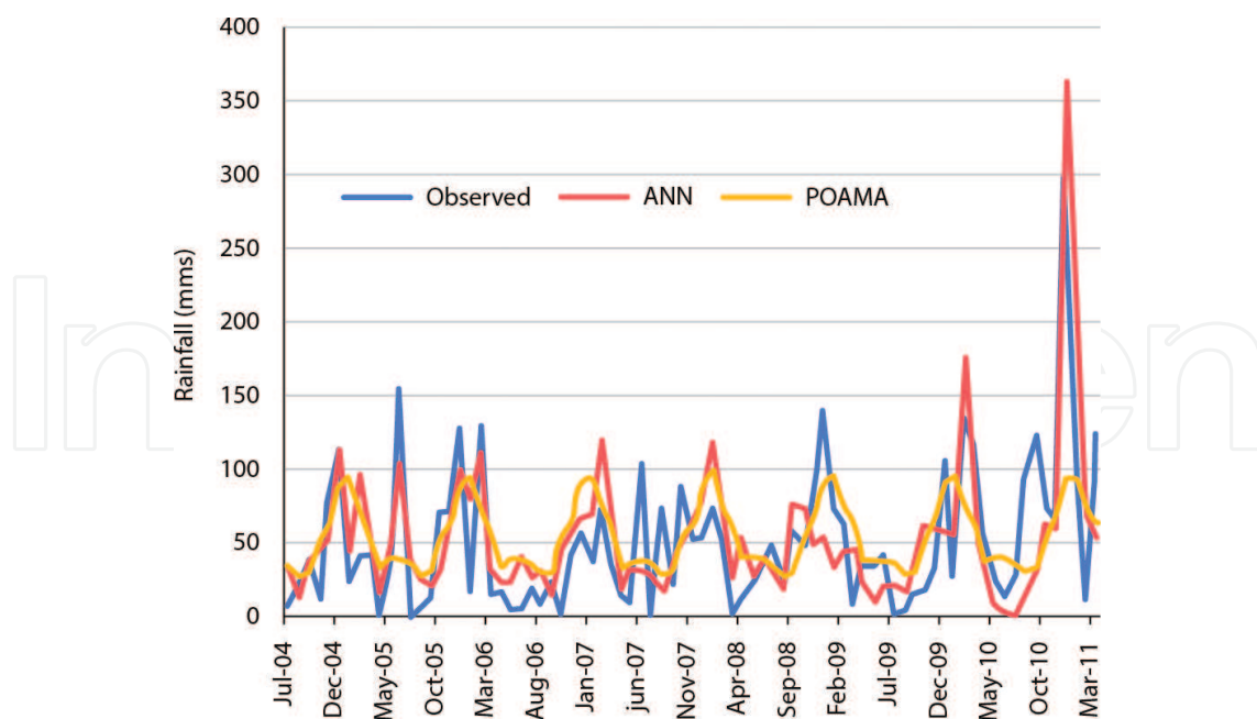
Figure 7. Forecasts for Miles from POAMA 1.5 (yellow line), and the ANN (red line) benchmarked against actual observed rainfall (blue line) for a 3-month lead for the period July 2004 to March 2011.
