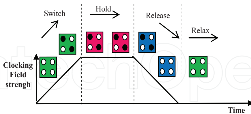
Figure 4. Schematic of interdot barriers in QCA clock.
