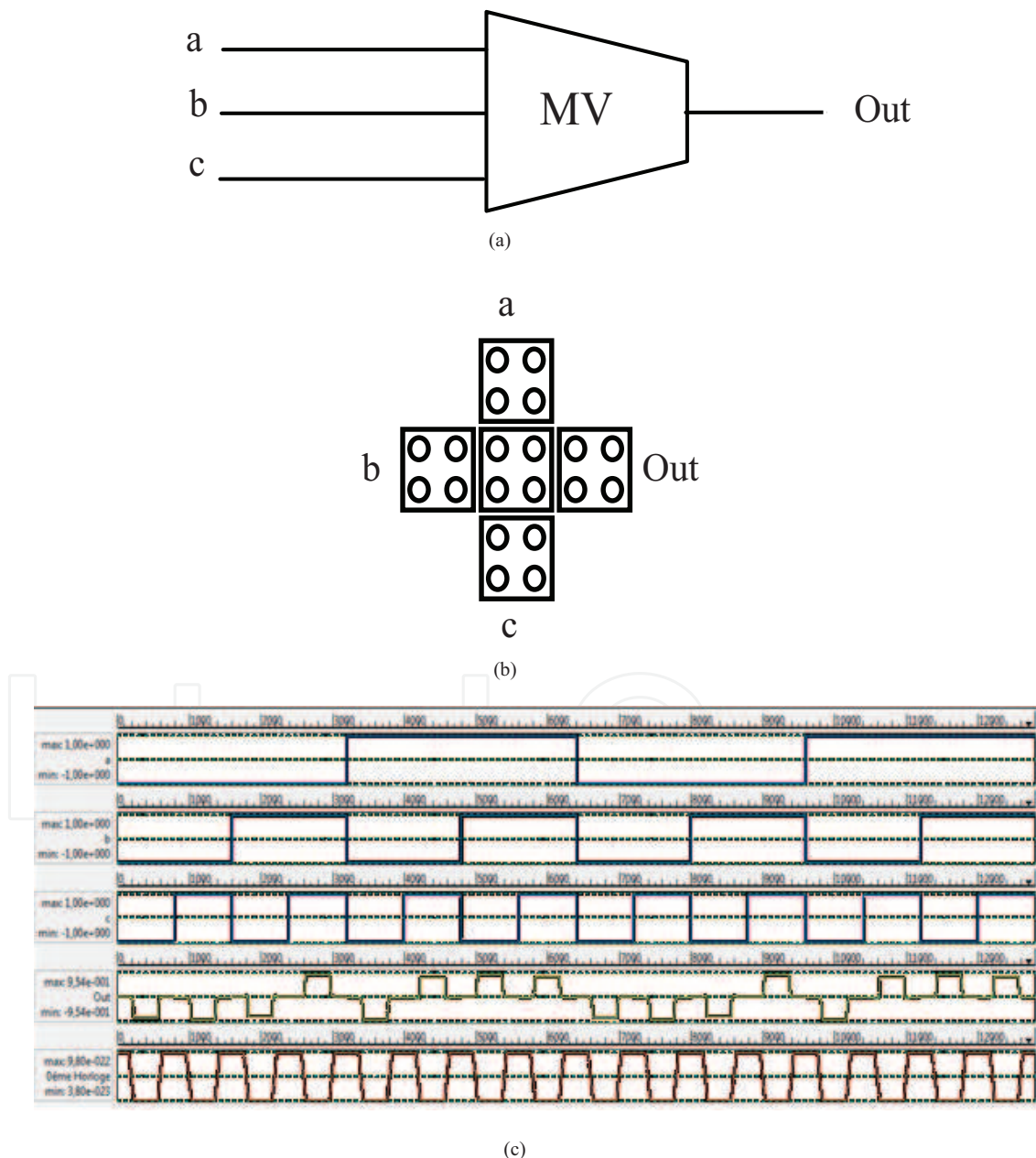
Figure 7. Majority voter (MV) gate, (a) QCA representation, (b) QCA layout, and (c) simulation results.
