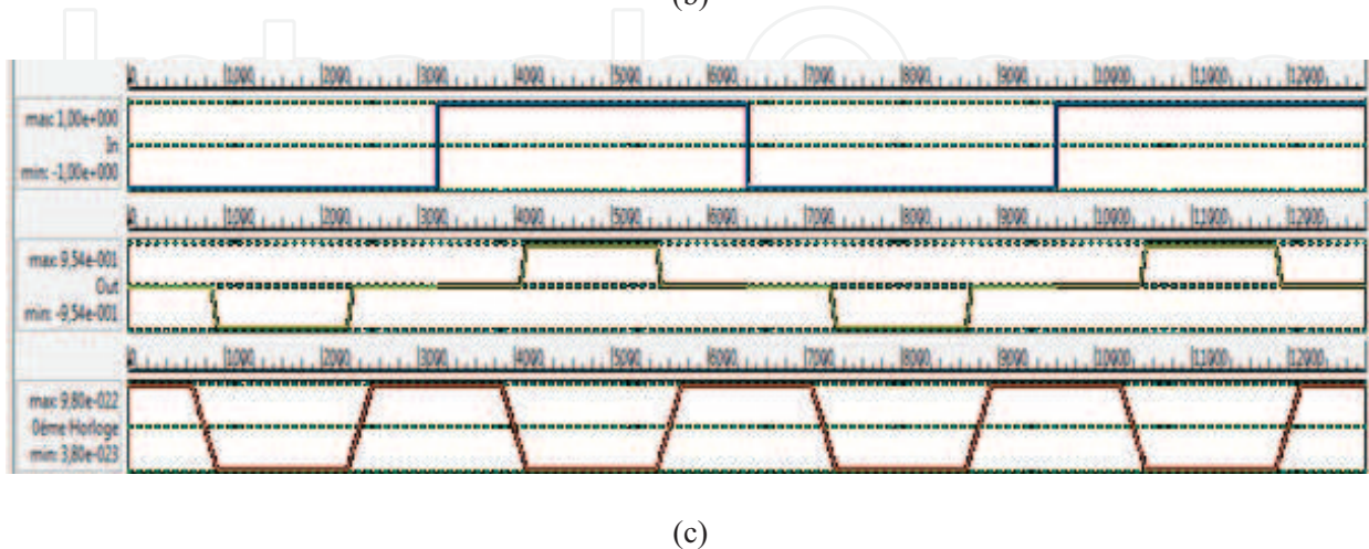
Figure 5. Binary wire, (a) representation, (b) QCA layout, and (c) simulation results.
