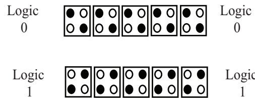
Figure 2. Operations of a QCA wire propagation by application of logic 0 and logic 1 to a QCA cell at the input.
