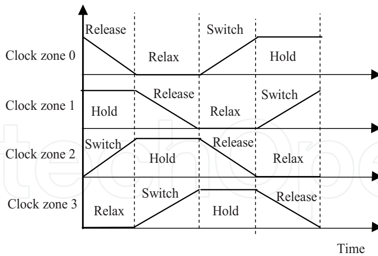
Figure 3. Four phases of QCA clock zones.
