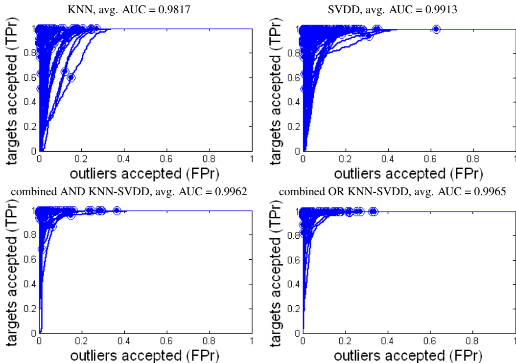
Figure 2: ROC of the 70 individual classifiers and their average AUC for each type of OCC considered and using feature trios.
