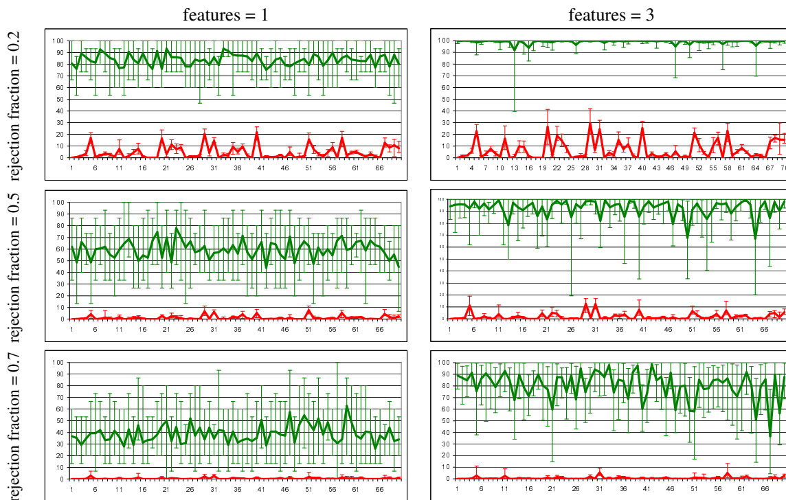
Figure 1: Average individual classification results of the combined OR KNN-SVDD classifier, obtained after 10 independent tests. The upper (green) curve in each graphic shows the average correct owner classifications per classifier, while the lower (red) curve shows the average false positives per classifier. The vertical line under each average value shows the maximum and minimum values observed in the 10 tests.
