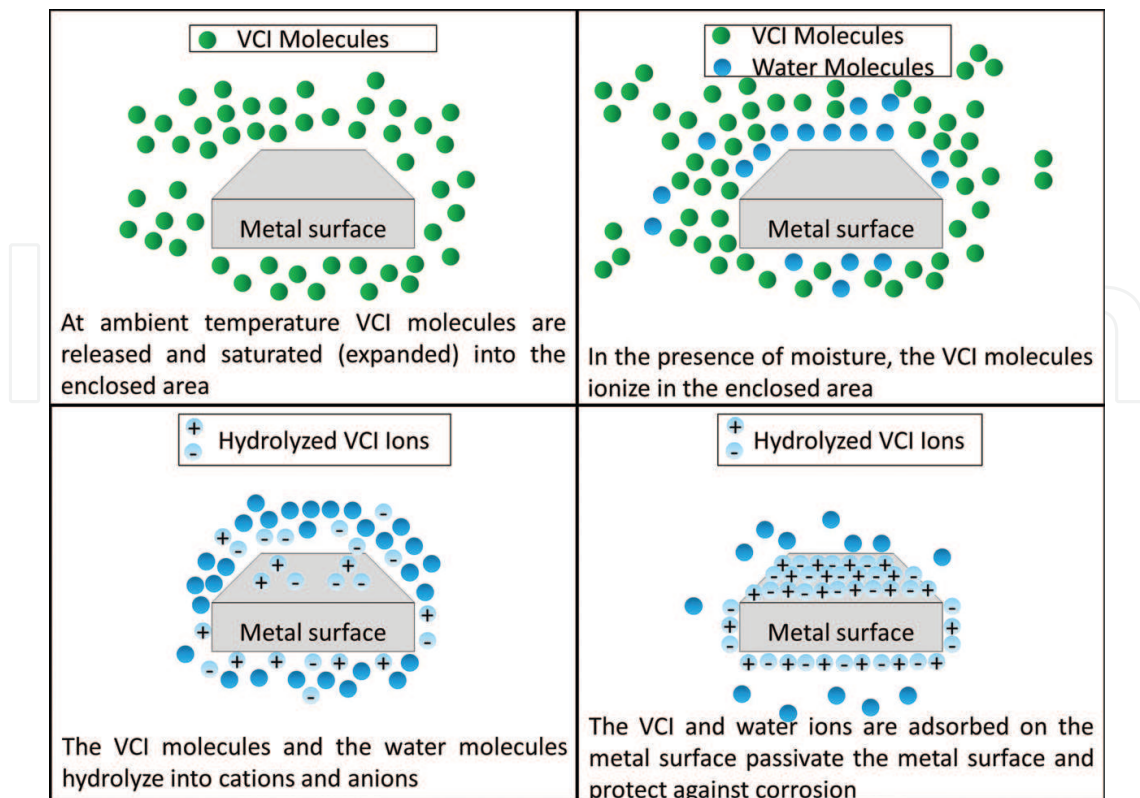
Figure 3. VCI molecule ionizes and hydrolyzes in the presence of moisture, forming a protective layer on the metal surface.
