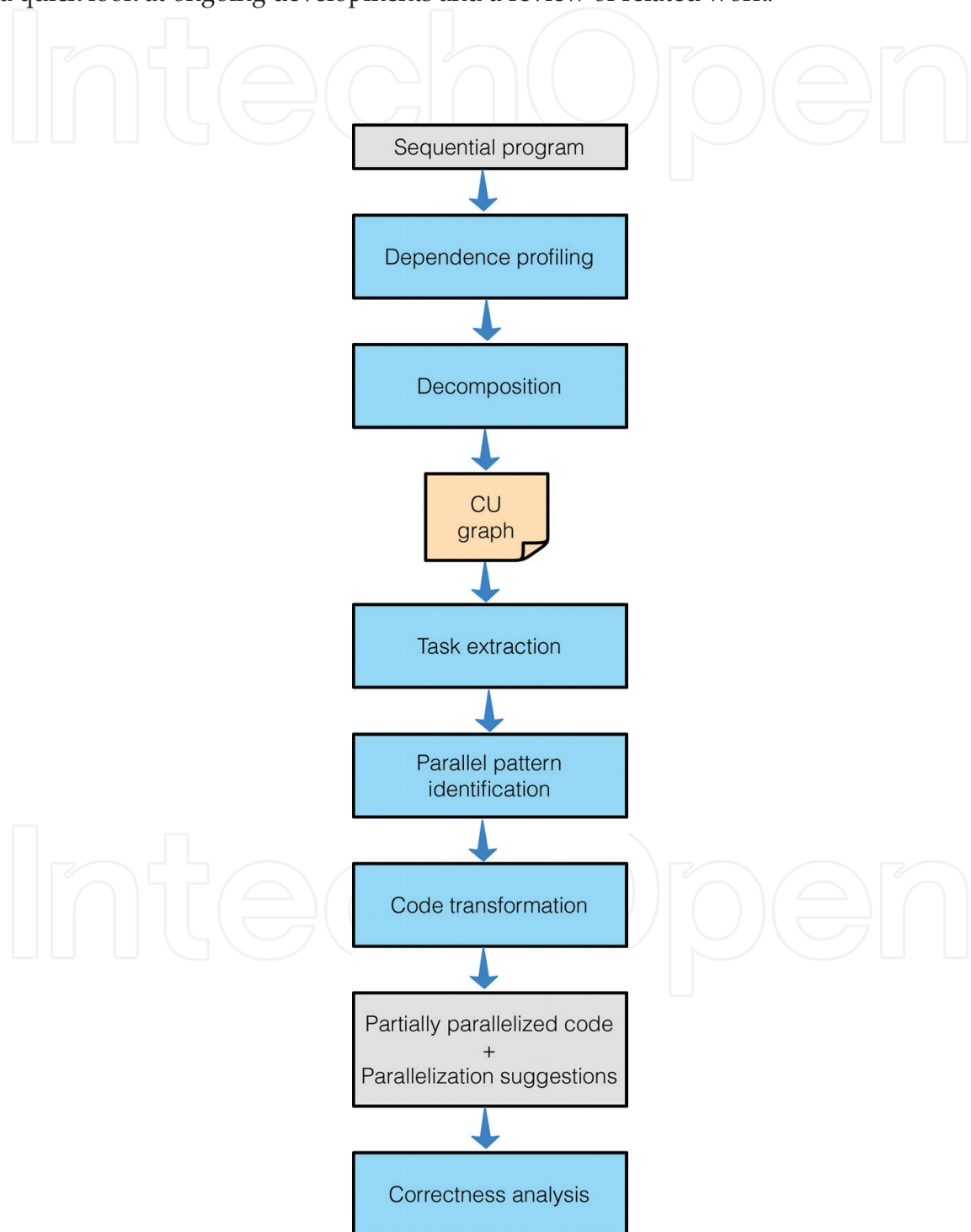
Figure 1. Main elements of the DiscoPoP parallelization approach.
