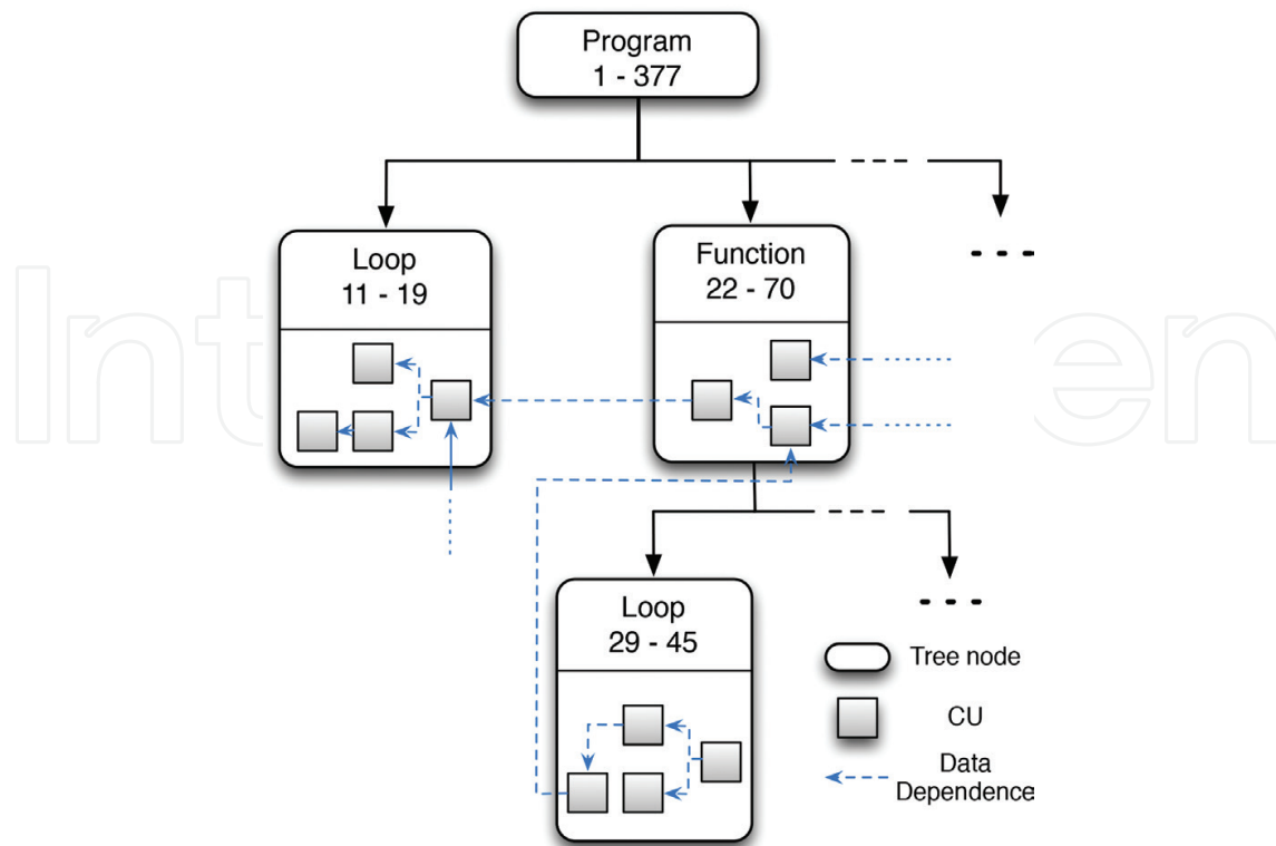
Figure 2. CU graph mapped onto the program execution tree.
