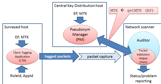
Fig. 2. Packet tagging architecture proposed in [1], where a traffic tagging application on a surveyed host shares a temporary pseudonym (EP) and a related master tagging key (MTK) with a Pseudonym Manager, and an authorized auditing application uses PM for getting the MTK given an EP
