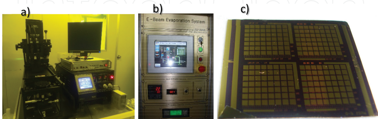
Figure 4. (a) Optical lithography. (b) E-Beam system. (c) Schematic of 2D final device fabrication with grids as a shadow mask with SiO 2 dielectric and Ti/Au electrodes.
