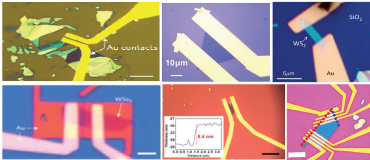
Figure 6. Optical and AFM images of different 2D devices gated using a degenerately doped silicon substrate with two gold contacts. Adapted from Lopez-Sanchez et al. [23], Xia et al. [101], Liu et al. [18], Baugher et al. [19], Huang et al. [20], Liu et al. [112].
