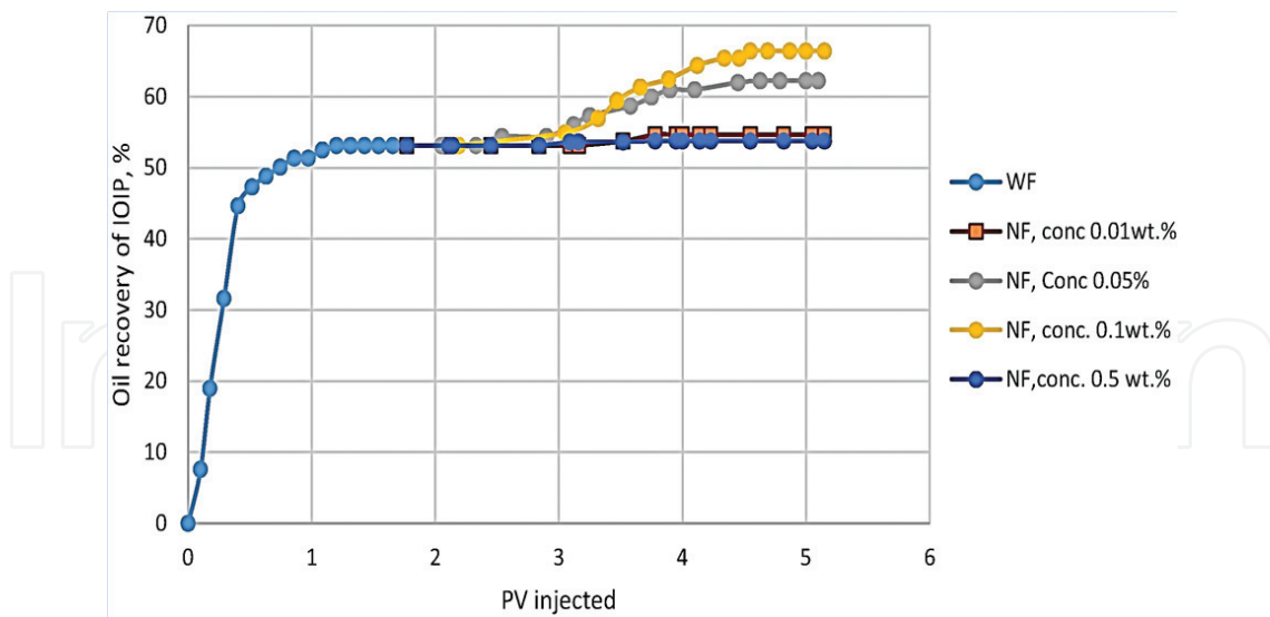
Figure 4. Oil recovery vs. pore volume (PV) injected for oil-wet Berea sandstone before and after nanofluid exposure [87].
