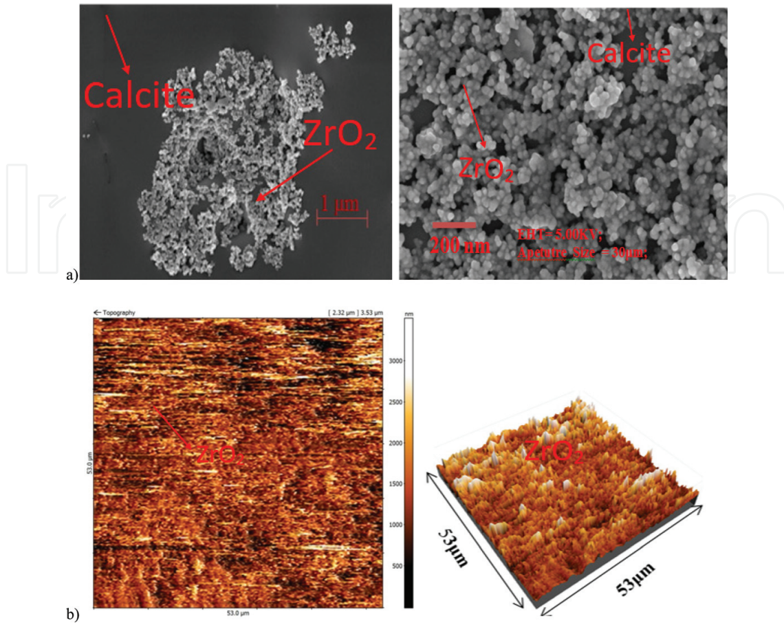
Figure 5. SEM (a) and AFM(b) images of ZrO_2 nanoparticle as uniform nano-spherical particle with mean particle size of 28 nm depicting surface adsorption on calcite substrates [23] © .
