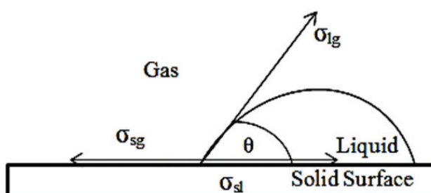
Figure 1. Young's equation illustrating a three-phase contact line.
