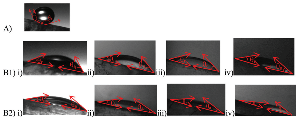
Figure 2. The receding ( \theta_r ) and advancing ( \theta_a ) contact angle images of water droplets (probe liquid) before and after exposure to nanofluid (A) oil modified rock (before nano-modification - high \theta - indicates the surface's hydrophobicity - 152^\circ \theta_a ); (B) nano modified at different temperatures (22–70°C) (B1- NiOC 16 TAB; B2 - ZrO 2 C 16 TAB - low \theta - indicates hydrophilic conditions) which represents strong interaction with the rock surface thus exhibiting low surface energies and inclination to wet; I-IV); see graphical representation (Figure 3) for \theta - values [24] © .
