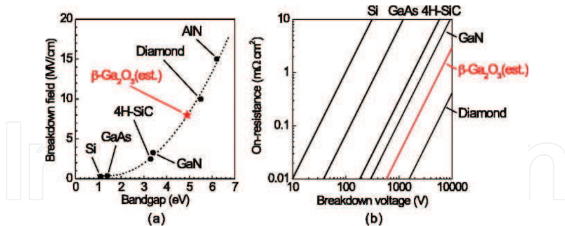
Figure 1. (a) Relationship between the bandgap and breakdown field for various semiconductor materials, (b) On-resistance as a function of breakdown voltage for major semiconductors. (Reprinted with permission from [82]. Copyright 2012, American Institute of Physics.)
