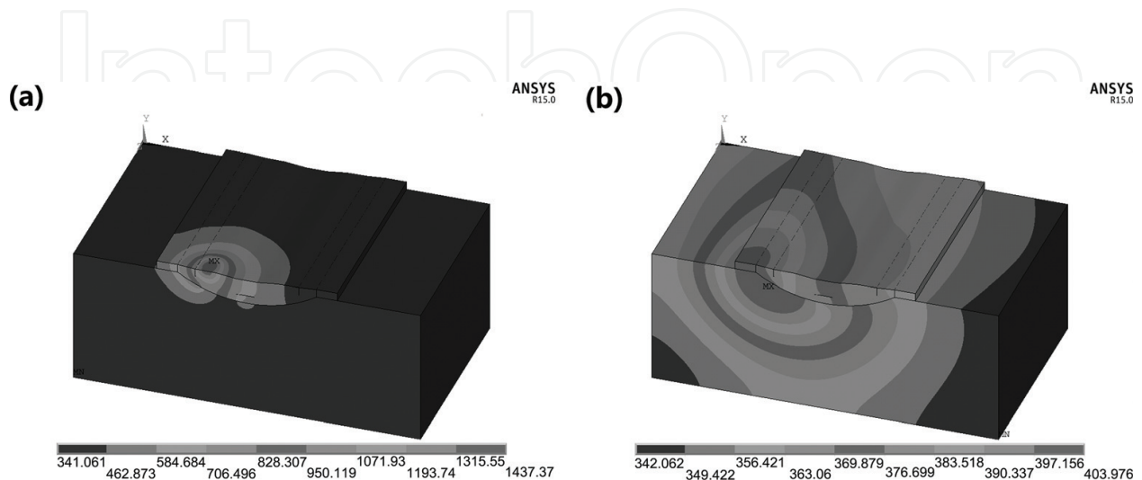
Figure 10. Temperature distribution at (a) 2 and (b) 5 s.
