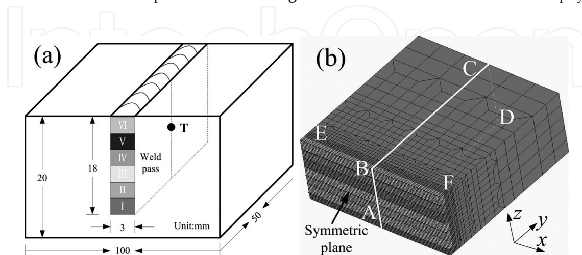
Figure 2. Sketch of the geometric model: (a) narrow gap groove and (b) mesh generation.
