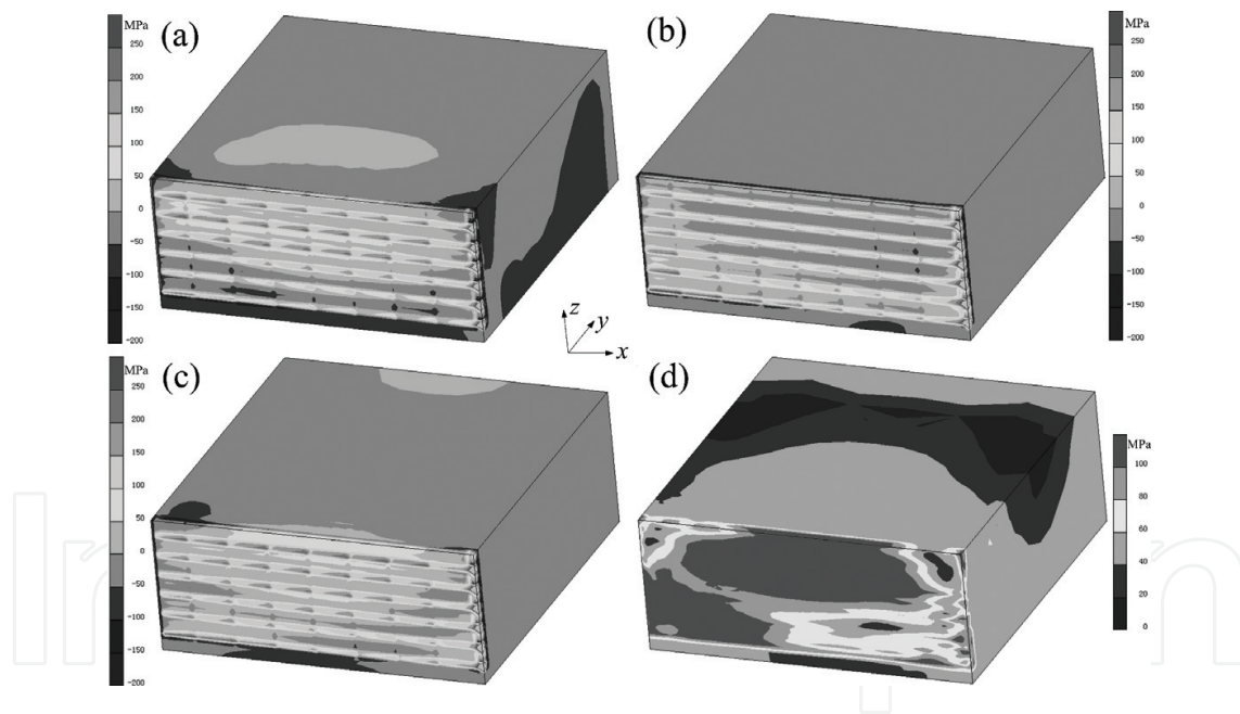
Figure 7. 3D residual stress distributions: (a) transverse residual stress \sigma_y (b) longitudinal residual stress \sigma_x (c) vertical residual stress \sigma_z and (d) von Mises equivalent stress.
