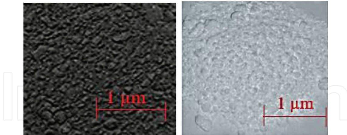
Figure 4. Nanoparticles in powder form (NiO-dark gray green color; ZrO 2 -white color).
