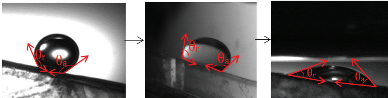
Figure 2. Rock surface wetting transition from hydrophobic to hydrophilic. Left: Oil-wet ( 105\text{--}180^\circ ); Center: Intermediate-wet ( 75\text{--}105^\circ ); right: Water-wet ( 0\text{--}75^\circ ).
