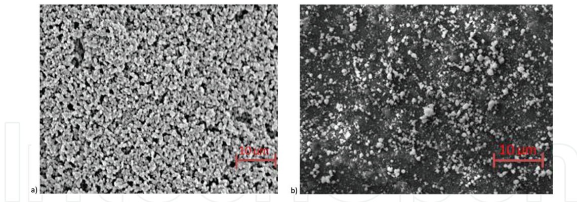
Figure 7. SEM images of: (a) \text{ZrO}_2 ; (b) NiO nanoparticles.
