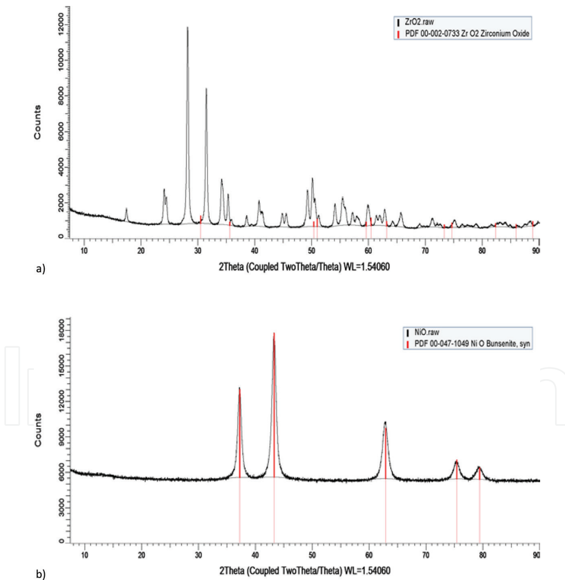
Figure 10. (a) Crystallographic phases of the \text{ZrO}_2 nanoparticles exhibiting tetragonal phase. (b). Crystallographic phase of the NiO nanoparticles exhibiting cubic phase.
