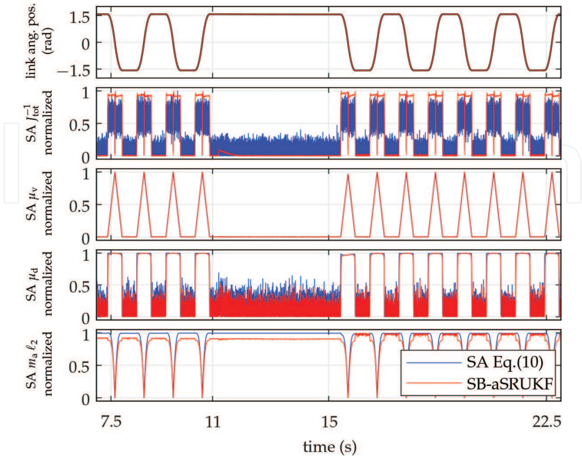
Figure 3. Sensitivity analysis (SA): comparison between the a posteriori state sensitivity obtained using the SB-aSRUKF and the resulting using Eq. (10). The desired link position was set as an s-curve between -\pi/2 and \pi/2 . The link position was held at \pi/2 after ca. 11 s for about 4.5 s. The parameter sensitivities are related to the link angular speed ( \hat{x}_2 = \hat{q}_1 ).
