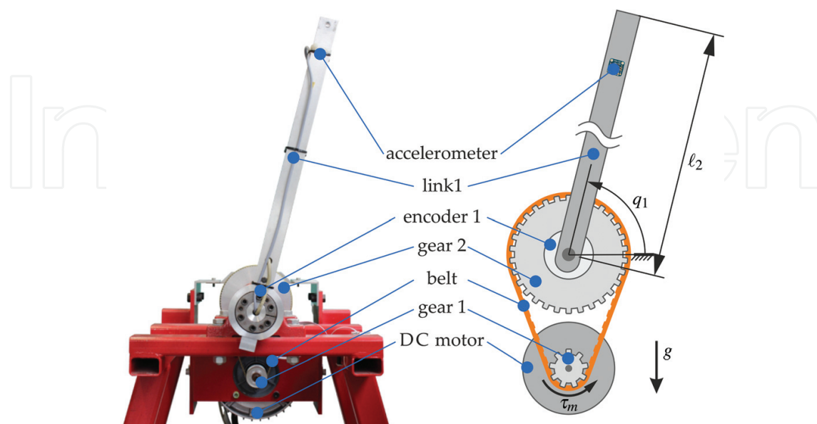
Figure 1. Planar one-link robot system: structure and functionality.
