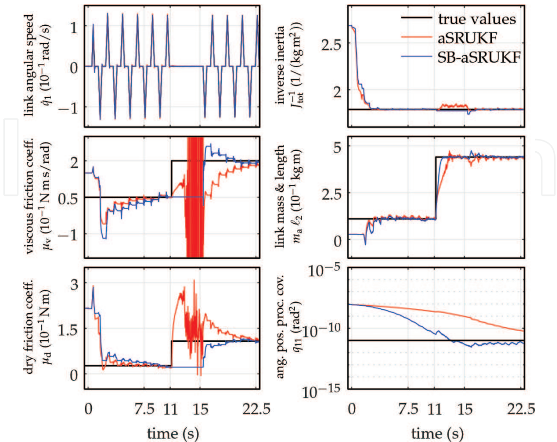
Figure 4. Planar one-link robot system: parameter and covariance estimation. The SB-aSRUKF uses SA to monitor the system excitation. The initial parameter \theta_{init} was randomly selected. The link position was held after ca. 11 s for about 4.5 s, and simultaneously the system parameters \hat{\mu}_v , \hat{\mu}_d , and \hat{m}_a were quadrupled.
