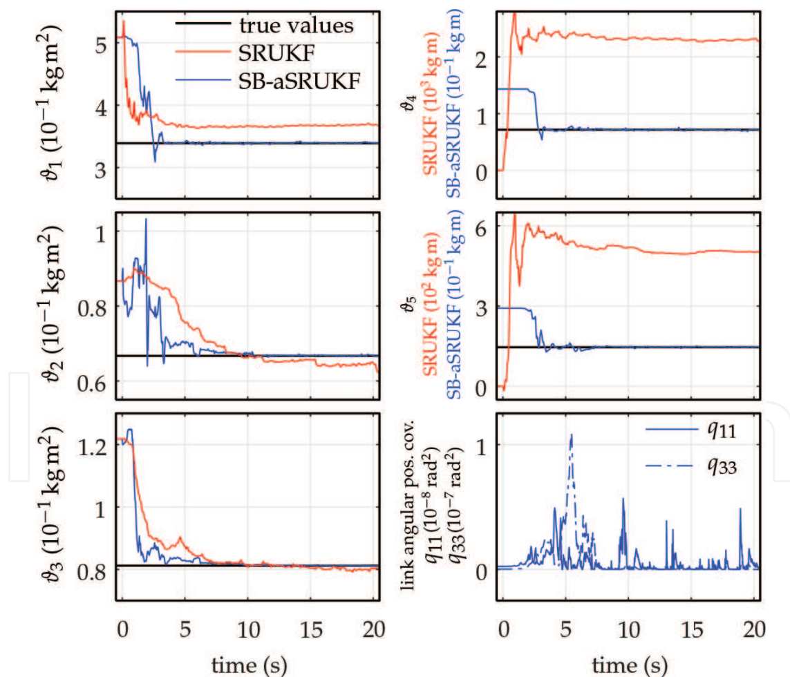
Figure 6. Pendubot: parameter and covariance estimation using the SB-aSRUKF and joint SRUKF. The SB-aSRUKF was configured to estimate the system parameters \vartheta_1 to \vartheta_5 and the process covariances corresponding to the link positions. The joint SRUKF estimates only the system parameters. It should be noted that the diagram scales for parameters \vartheta_4 and \vartheta_5 are different between the filters.
