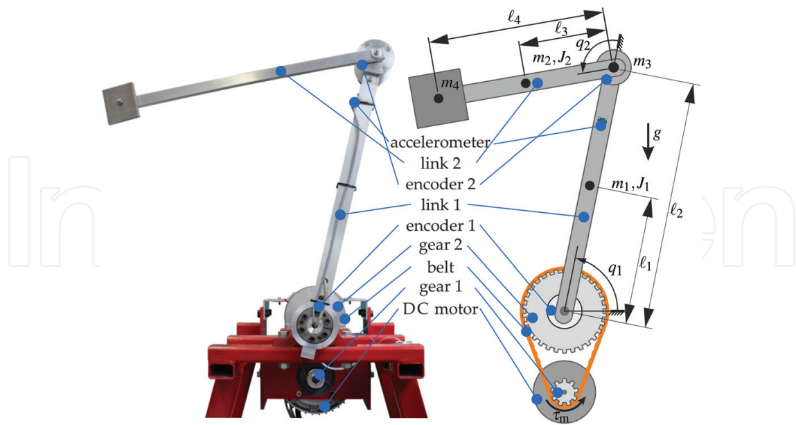
Figure 2. Pendubot: structure and functionality.
