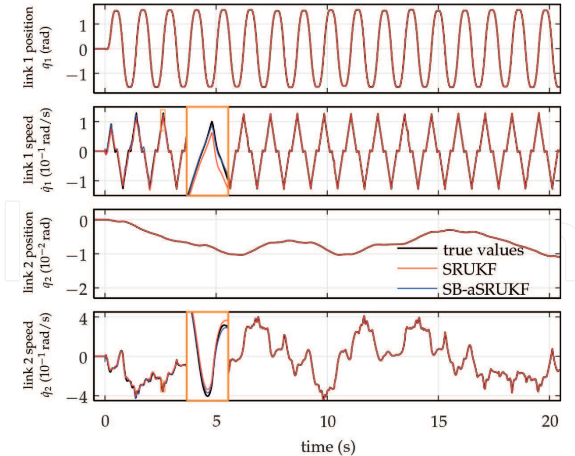
Figure 5. Pendubot: state estimation using the SB-aSRUKF and joint SRUKF. Both filters followed the dynamic of the true system states without any significant bias.
