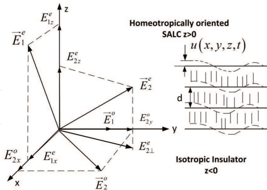
Figure 4. The polarizations of the fundamental ordinary waves \vec{E}_{1,2}^o and extraordinary waves \vec{E}_{1,2}^e in SALC ( z > 0 ).
