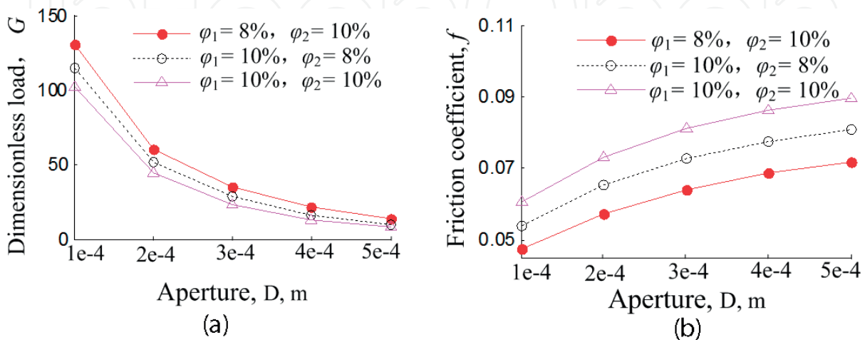
Figure 5. Effect of pore structure on oil slick bearing capacity and friction coefficient.
