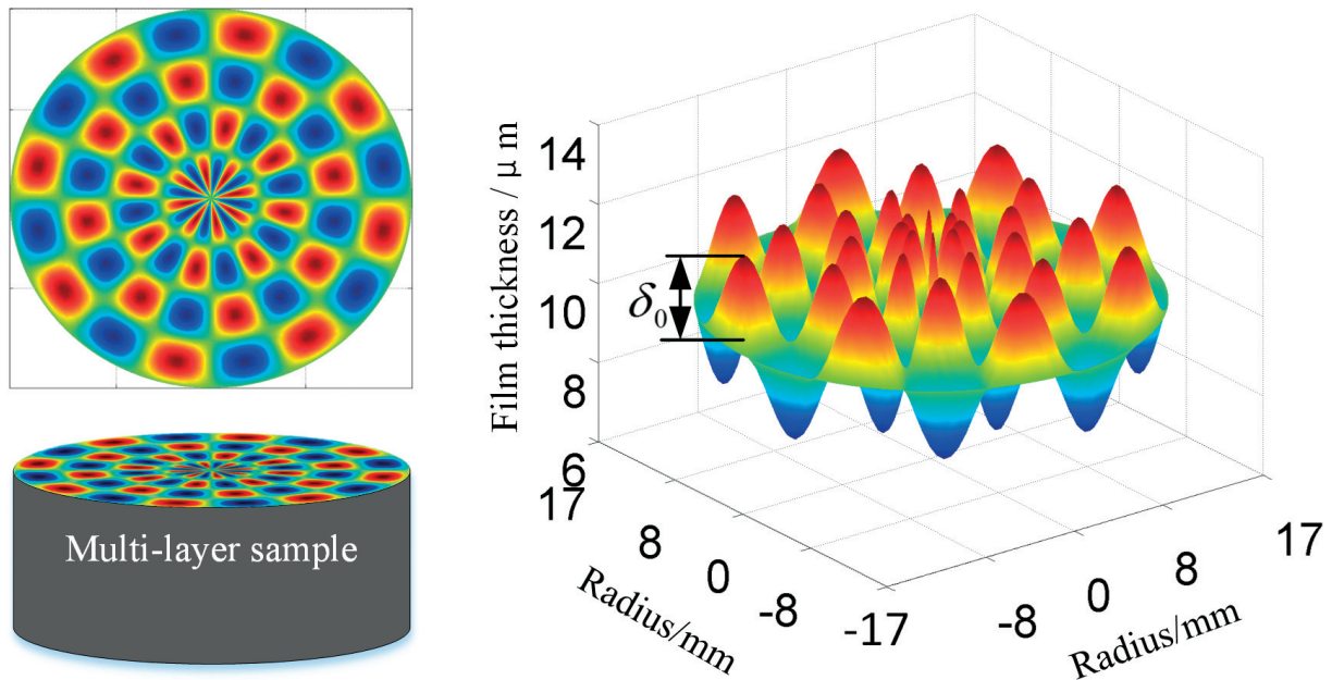
Figure 2. Film thickness.
