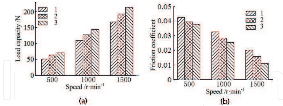
Figure 4. Effect of surface Darcy flow on the friction coefficient in different speeds. (a) Carrying capacity (b) Friction coefficient. Note: 1 denote monolayer material ignored Darcy flow; 2 denote multi-layer material ignored Darcy flow; 3 denote multi-layer material included Darcy flow.
