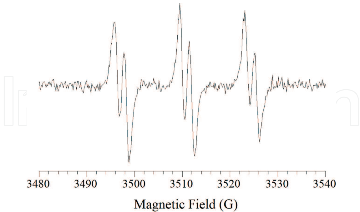
Figure 1. EPR spectrum of PBN adduct of radicals extracted from Podarcis sicula testis.
