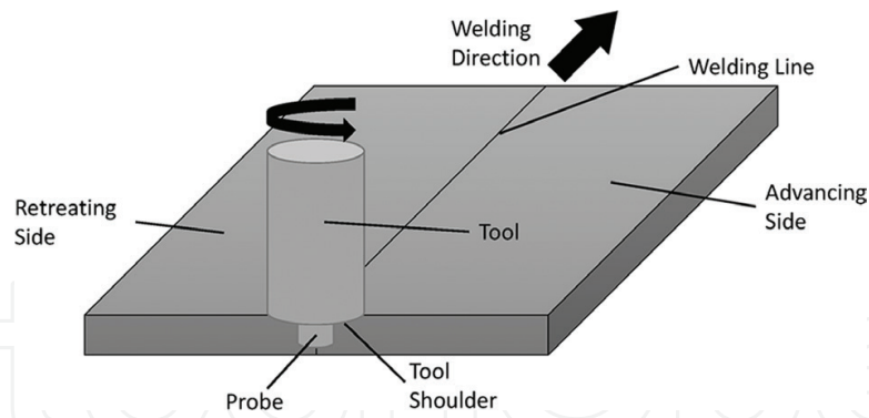
Figure 1. Scheme of friction stir welding process.
