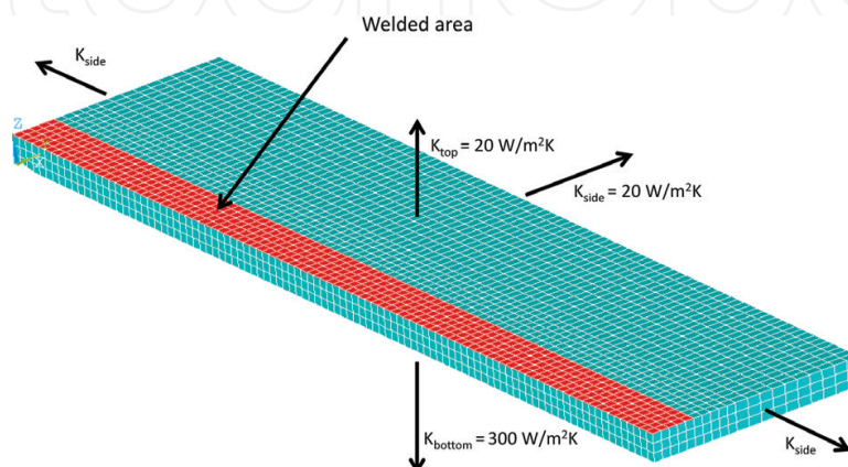
Figure 5. FSW model mesh and convection coefficient.
