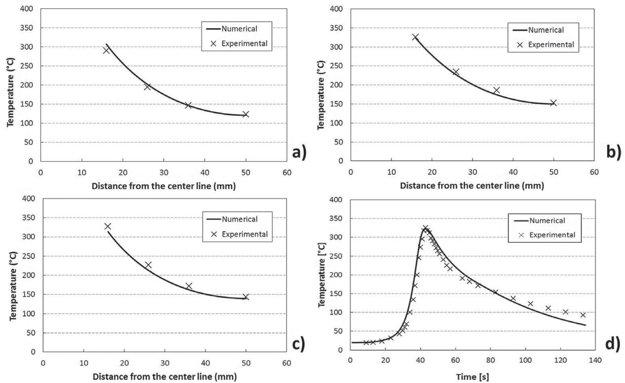
Figure 8. Temperature trend in the start phase (a), in the middle phase (b) and in the end phase (c) and temperature vs. time of a middle point distant 16 mm from the centre line (d) for FSW.
