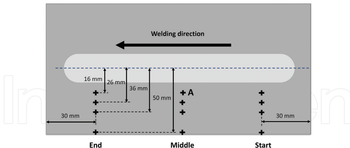
Figure 7. Location scheme of experimental measured points.
