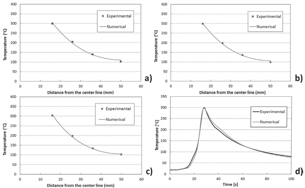
Figure 11. Temperature trend in the start phase (a), in the middle phase (b) and in the end phase (c) and temperature vs. time of a middle point distant 16 mm from the centre line (d) for LAFSW.
