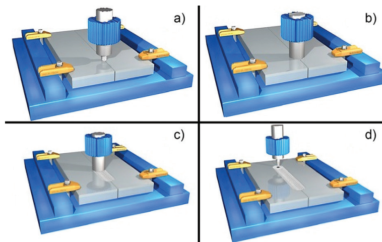
Figure 2. Scheme of FSW process steps: (a) rotating tool before plunging, (b) plunging and then tool shoulder touches the work piece producing frictional heat, (c) rotating tool traverses along the work piece and (d) pulling out from the workpiece.
