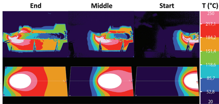
Figure 9. Graphical comparison between numerical data and the experimental ones for FSW.
