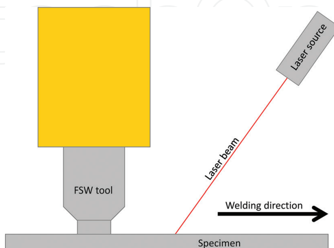
Figure 3. Scheme of the LAFSW setup.
