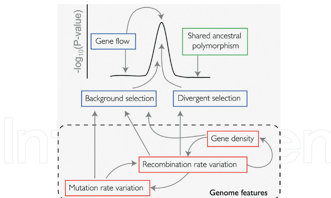
Figure 2. Multiple causes explain genome-environment associations. External processes, such as divergent selection, which is the main focus when assessing adaptation in wild relatives and landraces of crops, is only one of many possible causes. At the same time, the genomic background may be homogenized by gene flow [26]. Similarly, background selection and genomic features in regions of reduced recombination rate and shared ancestral polymorphism (more prone to genetic drift due to their reduced effective population size) could induce hotspots of spurious genome-environment associations. Therefore, besides external processes driven by natural selection, both inherent properties of the genome and the demographic and evolutionary history of the crop influence the extent of the genome-environment associations. Modified from Ravinet, Faria [64].
