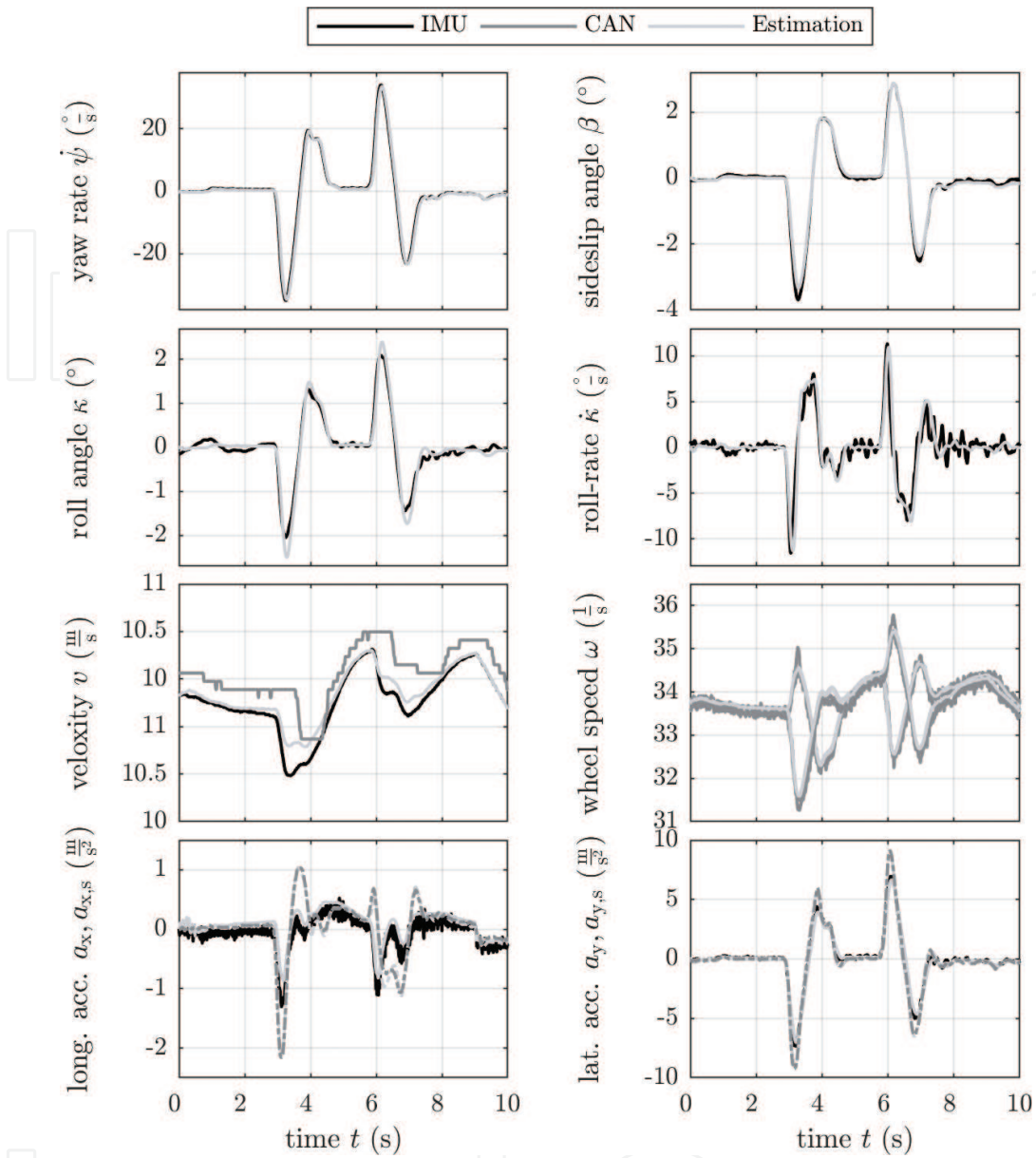
Figure 7. Vehicle state estimation during double-lane change maneuver.
