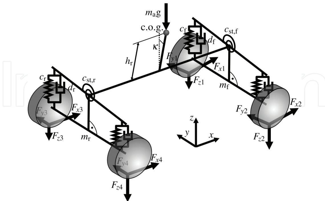
Figure 1. Two-track model including roll dynamics of a vehicle performing a left turn.
